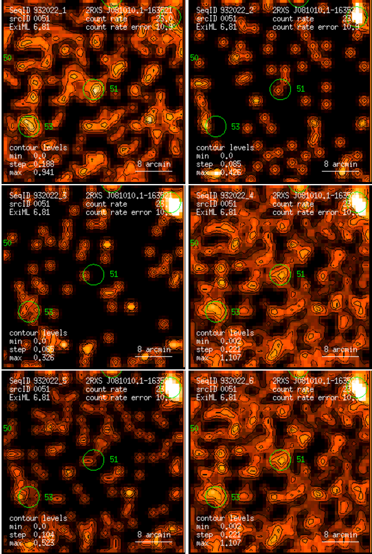
Figure 51: RASS 932022: detection 0051: band rate images, Gaussian filter: (1) PSPC channels 11 – 41, (2) 52 – 90, (3) 91 – 201, (4) 11 – 235, (5) 52 – 201, (6) 11 – 201. Broad band rates in counts/ks. Band rate contour levels in counts/ks/arcmin 2 .
