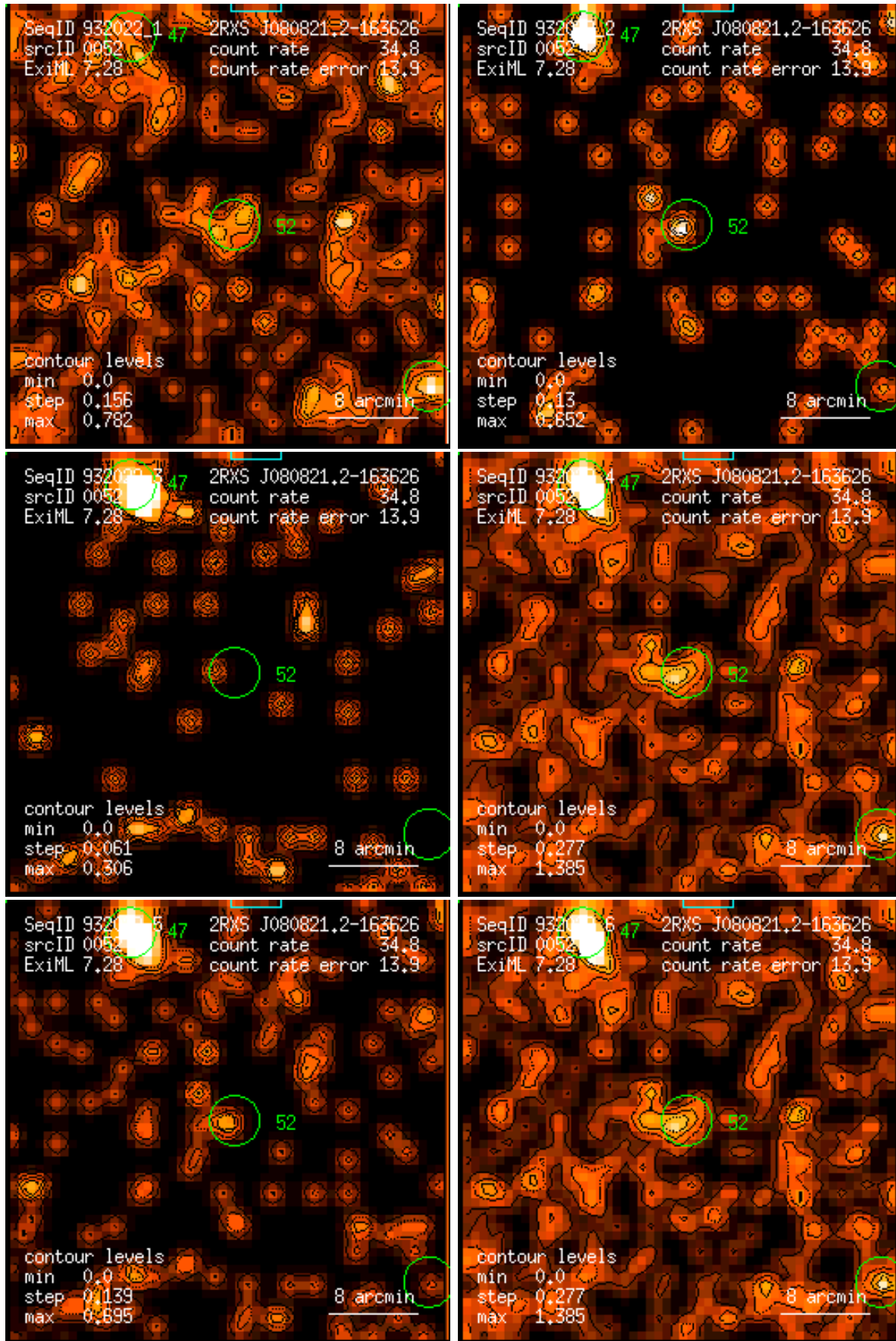
Figure 52: RASS 932022: detection 0052: band rate images, Gaussian filter: (1) PSPC channels 11 – 41, (2) 52 – 90, (3) 91 – 201, (4) 11 – 235, (5) 52 – 201, (6) 11 – 201. Broad band rates in counts/ks. Band rate contour levels in counts/ks/arcmin 2 .
