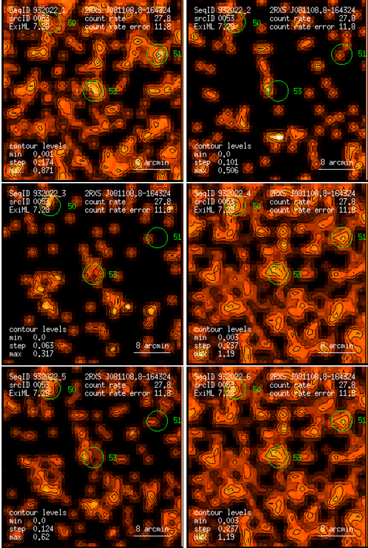
Figure 53: RASS 932022: detection 0053: band rate images, Gaussian filter: (1) PSPC channels 11 – 41, (2) 52 – 90, (3) 91 – 201, (4) 11 – 235, (5) 52 – 201, (6) 11 – 201. Broad band rates in counts/ks. Band rate contour levels in counts/ks/arcmin 2 .
