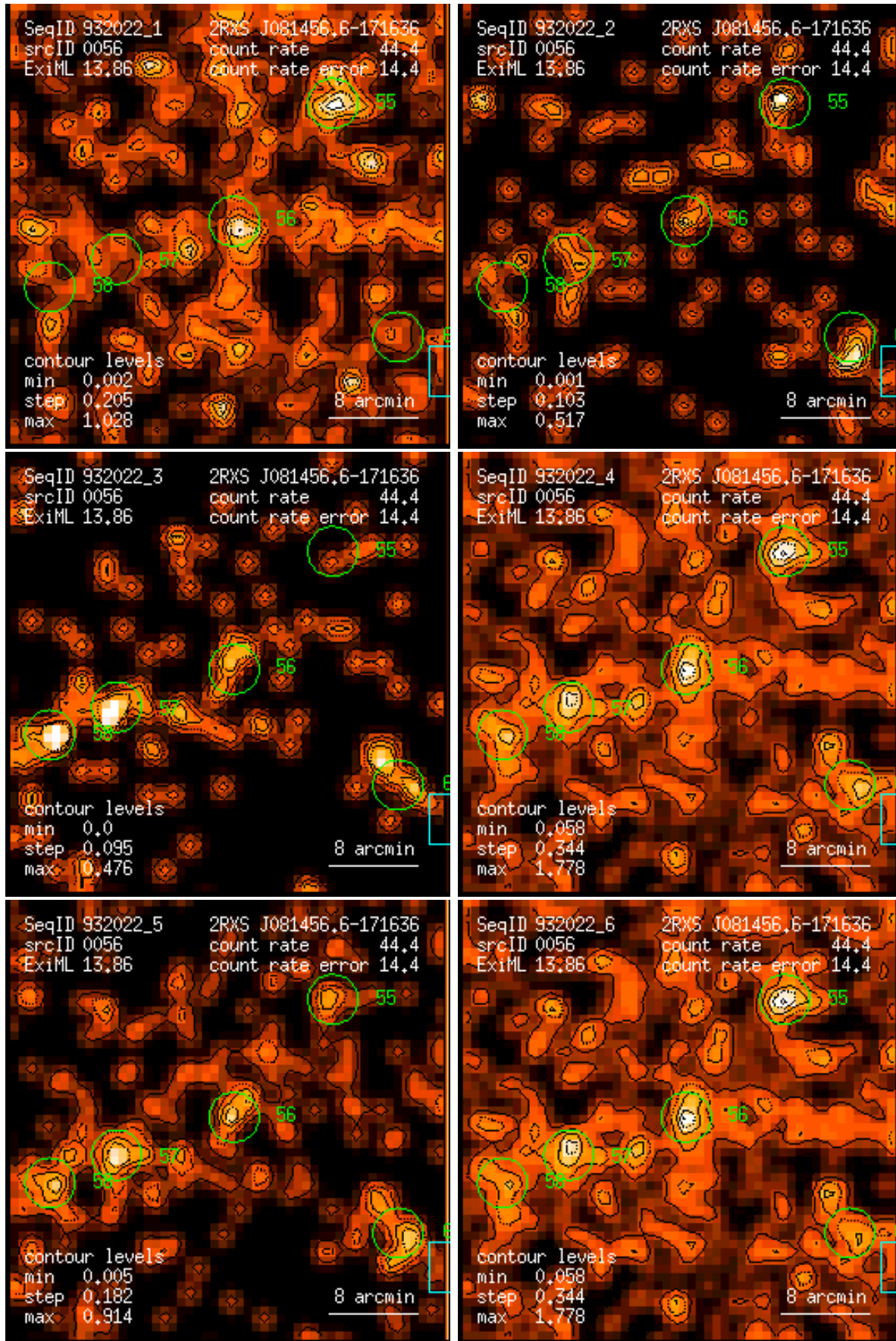
Figure 56: RASS 932022: detection 0056: band rate images, Gaussian filter: (1) PSPC channels 11 – 41, (2) 52 – 90, (3) 91 – 201, (4) 11 – 235, (5) 52 – 201, (6) 11 – 201. Broad band rates in counts/ks. Band rate contour levels in counts/ks/arcmin 2 .
