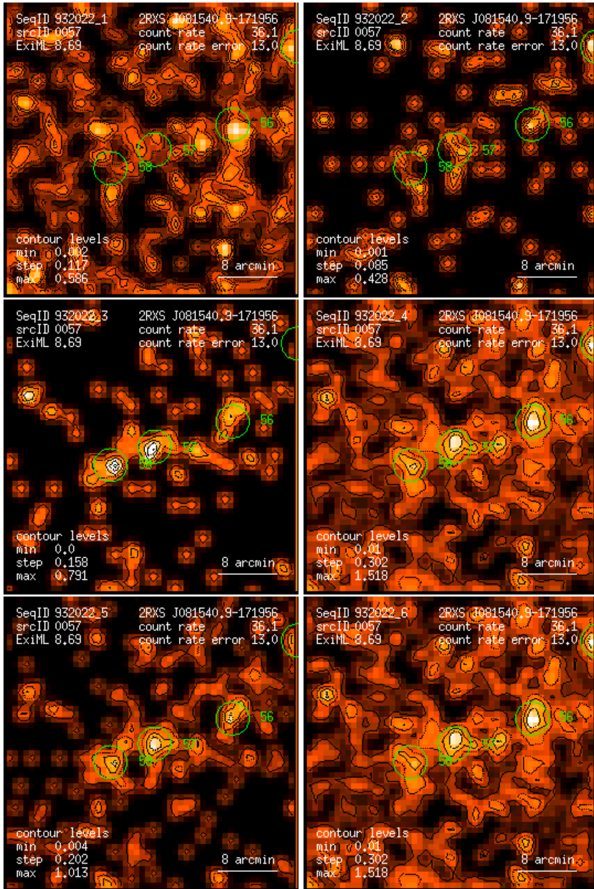
Figure 57: RASS 932022: detection 0057: band rate images, Gaussian filter: (1) PSPC channels 11 – 41, (2) 52 – 90, (3) 91 – 201, (4) 11 – 235, (5) 52 – 201, (6) 11 – 201. Broad band rates in counts/ks. Band rate contour levels in counts/ks/arcmin 2 .
