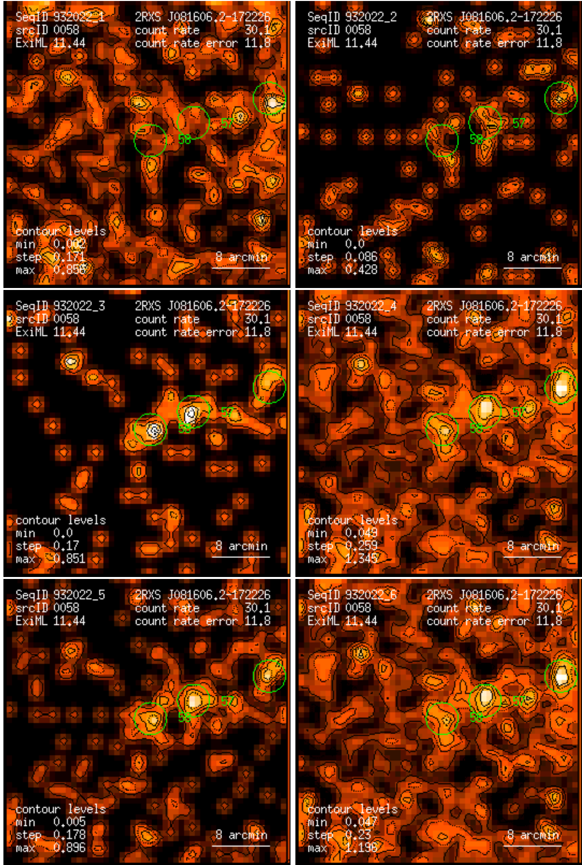
Figure 58: RASS 932022: detection 0058: band rate images, Gaussian filter: (1) PSPC channels 11 – 41, (2) 52 – 90, (3) 91 – 201, (4) 11 – 235, (5) 52 – 201, (6) 11 – 201. Broad band rates in counts/ks. Band rate contour levels in counts/ks/arcmin 2 .
