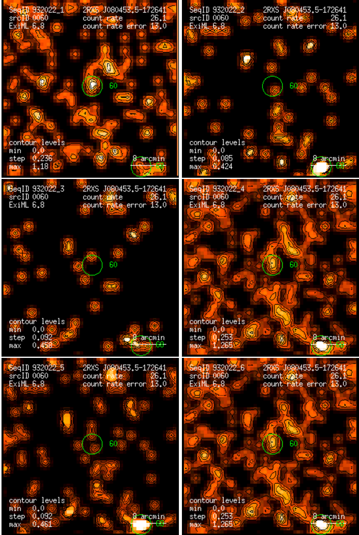
Figure 60: RASS 932022: detection 0060: band rate images, Gaussian filter: (1) PSPC channels 11 – 41, (2) 52 – 90, (3) 91 – 201, (4) 11 – 235, (5) 52 – 201, (6) 11 – 201. Broad band rates in counts/ks. Band rate contour levels in counts/ks/arcmin 2 .
