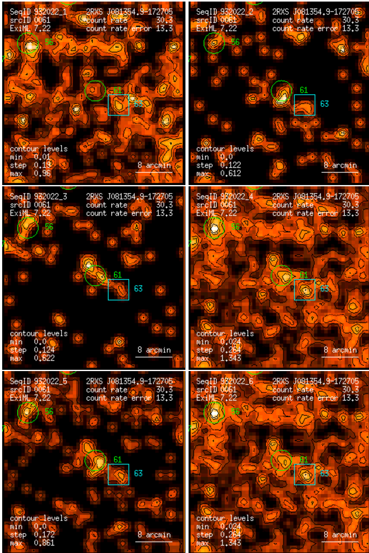
Figure 61: RASS 932022: detection 0061: band rate images, Gaussian filter: (1) PSPC channels 11 – 41, (2) 52 – 90, (3) 91 – 201, (4) 11 – 235, (5) 52 – 201, (6) 11 – 201. Broad band rates in counts/ks. Band rate contour levels in counts/ks/arcmin 2 .
