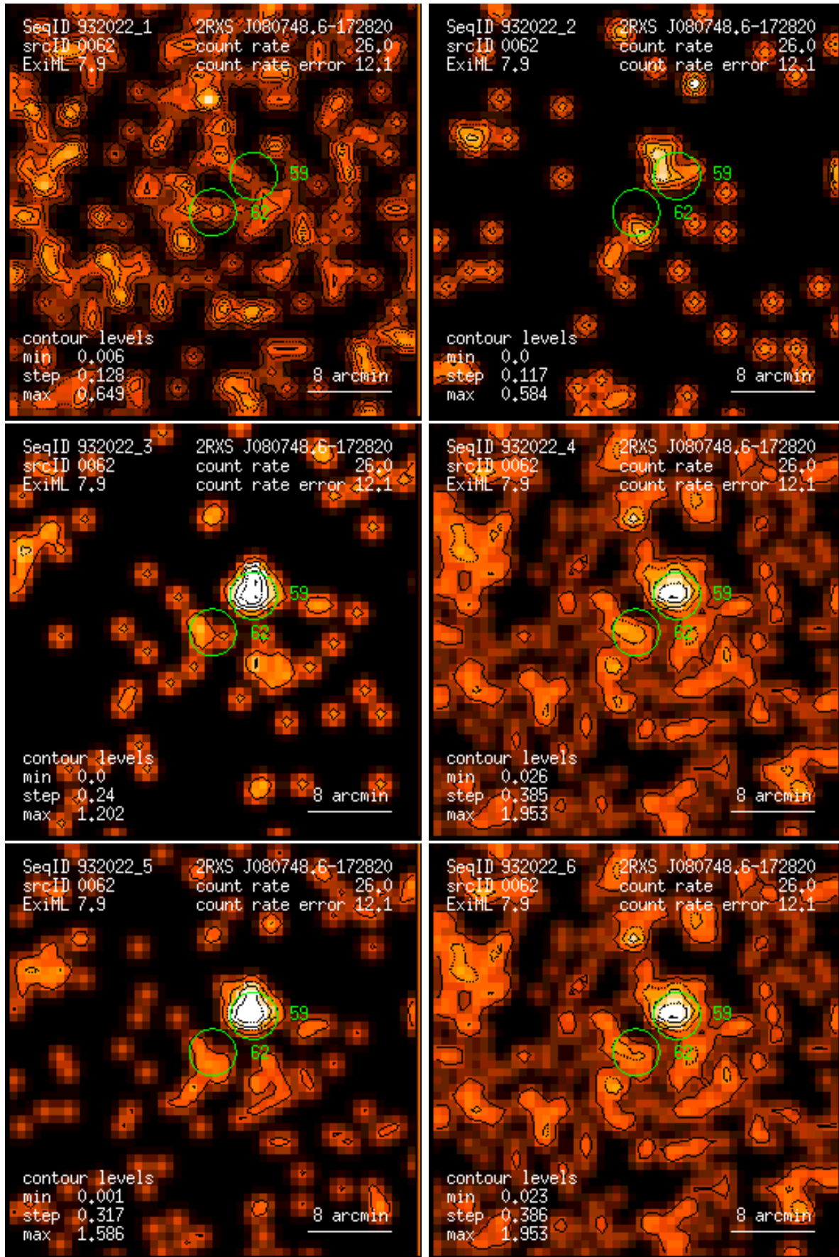
Figure 62: RASS 932022: detection 0062: band rate images, Gaussian filter: (1) PSPC channels 11 – 41, (2) 52 – 90, (3) 91 – 201, (4) 11 – 235, (5) 52 – 201, (6) 11 – 201. Broad band rates in counts/ks. Band rate contour levels in counts/ks/arcmin 2 .
