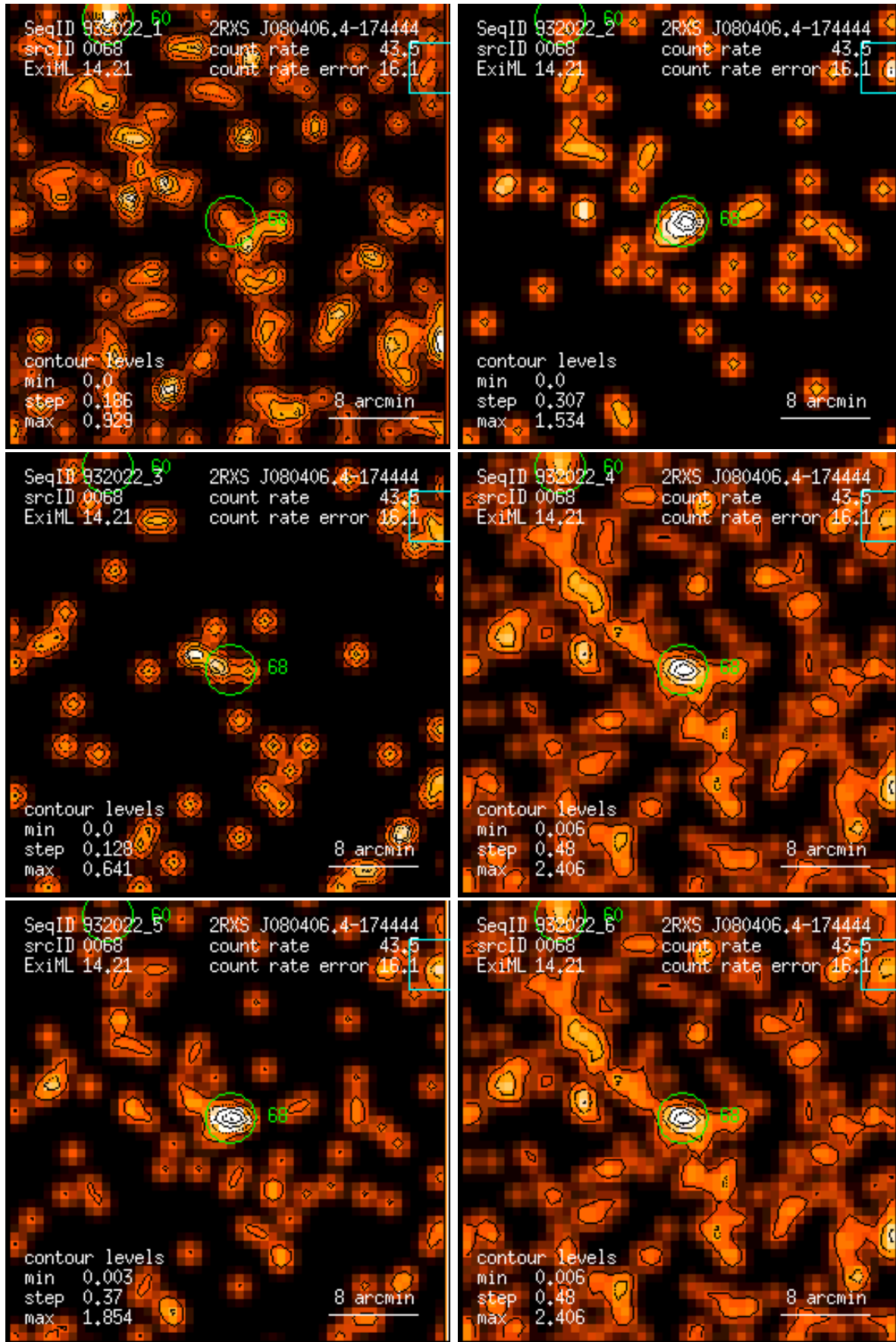
Figure 68: RASS 932022: detection 0068: band rate images, Gaussian filter: (1) PSPC channels 11 – 41, (2) 52 – 90, (3) 91 – 201, (4) 11 – 235, (5) 52 – 201, (6) 11 – 201. Broad band rates in counts/ks. Band rate contour levels in counts/ks/arcmin 2 .
