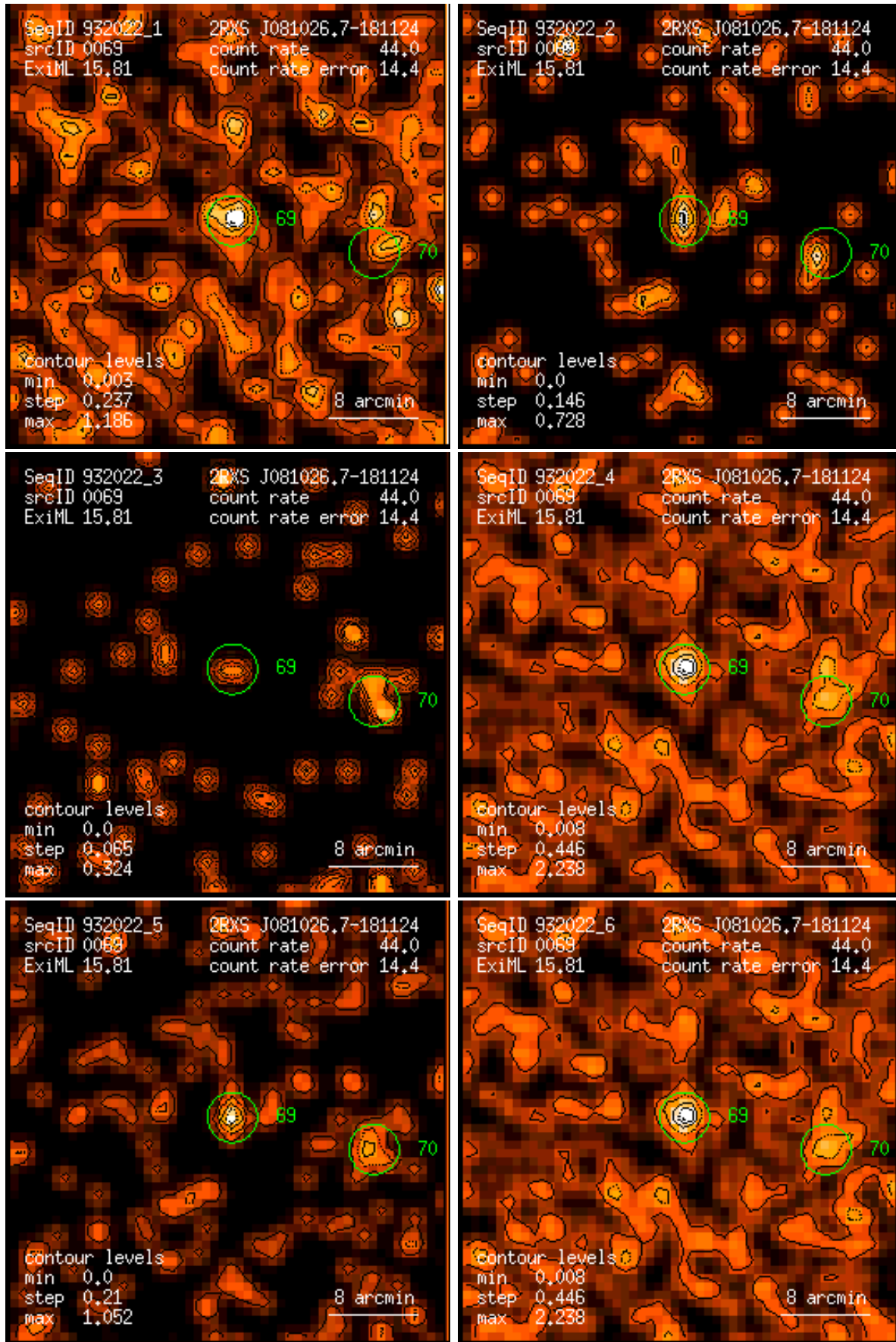
Figure 69: RASS 932022: detection 0069: band rate images, Gaussian filter: (1) PSPC channels 11 – 41, (2) 52 – 90, (3) 91 – 201, (4) 11 – 235, (5) 52 – 201, (6) 11 – 201. Broad band rates in counts/ks. Band rate contour levels in counts/ks/arcmin 2 .
