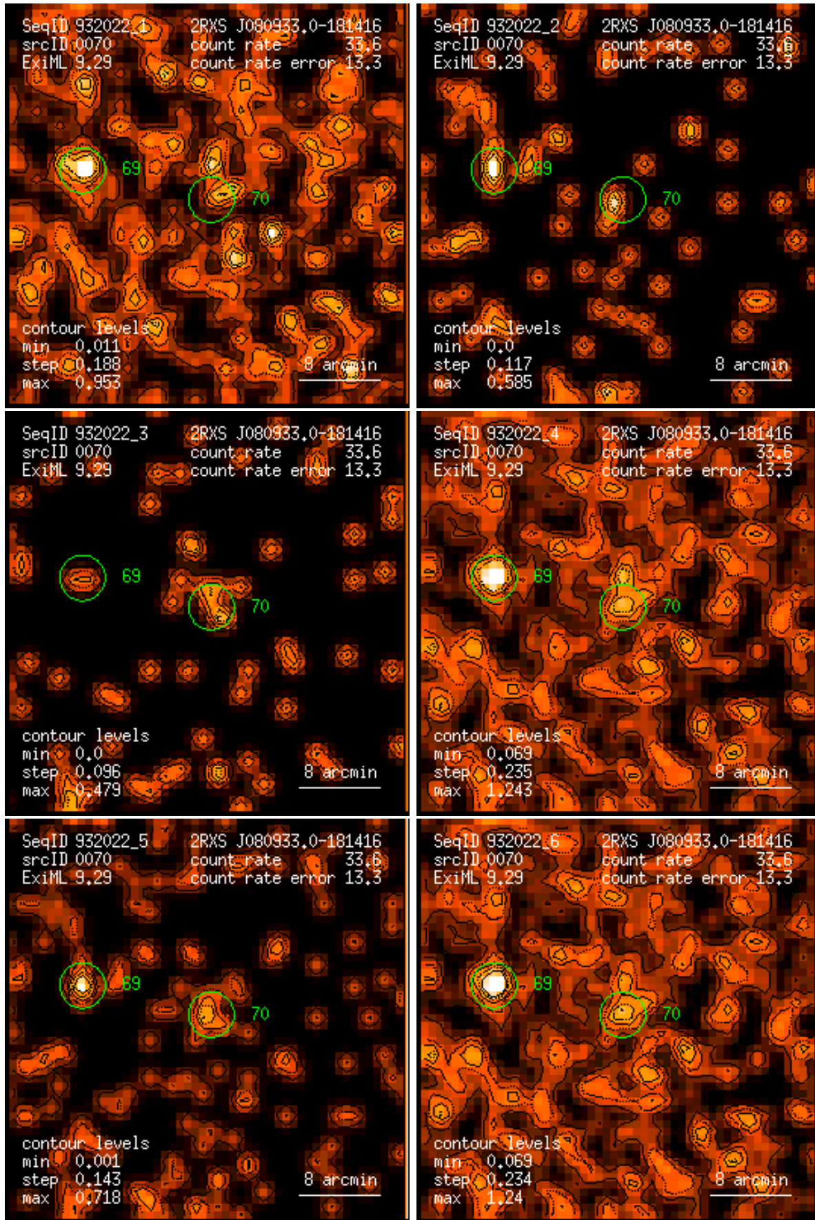
Figure 70: RASS 932022: detection 0070: band rate images, Gaussian filter: (1) PSPC channels 11 – 41, (2) 52 – 90, (3) 91 – 201, (4) 11 – 235, (5) 52 – 201, (6) 11 – 201. Broad band rates in counts/ks. Band rate contour levels in counts/ks/arcmin 2 .
