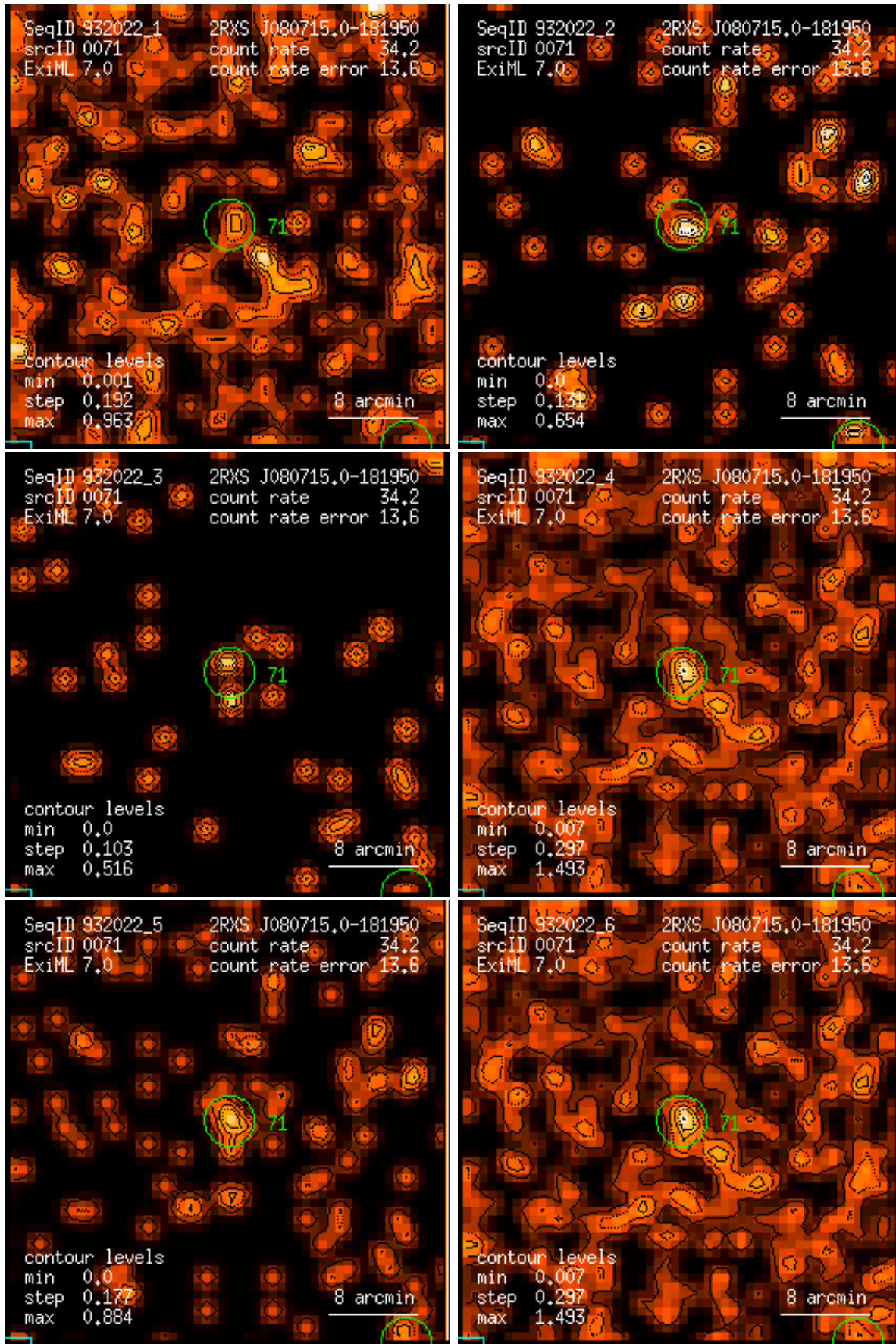
Figure 71: RASS 932022: detection 0071: band rate images, Gaussian filter: (1) PSPC channels 11 – 41, (2) 52 – 90, (3) 91 – 201, (4) 11 – 235, (5) 52 – 201, (6) 11 – 201. Broad band rates in counts/ks. Band rate contour levels in counts/ks/arcmin 2 .
