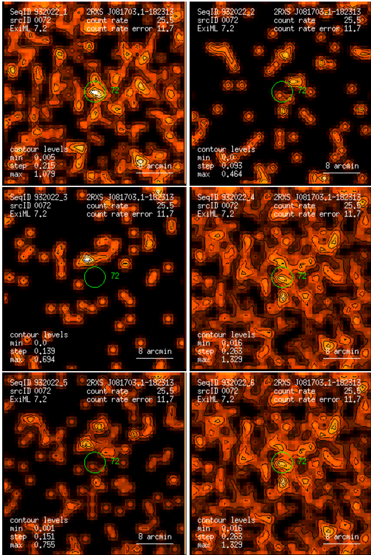
Figure 72: RASS 932022: detection 0072: band rate images, Gaussian filter: (1) PSPC channels 11 – 41, (2) 52 – 90, (3) 91 – 201, (4) 11 – 235, (5) 52 – 201, (6) 11 – 201. Broad band rates in counts/ks. Band rate contour levels in counts/ks/arcmin 2 .
