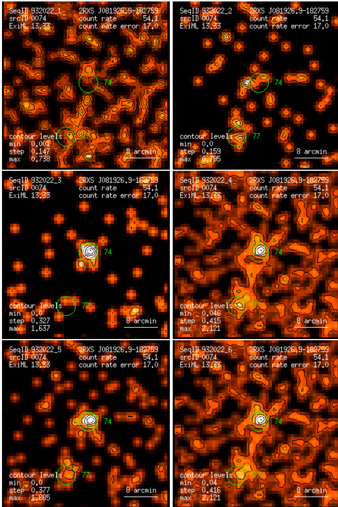
Figure 74: RASS 932022: detection 0074: band rate images, Gaussian filter: (1) PSPC channels 11 – 41, (2) 52 – 90, (3) 91 – 201, (4) 11 – 235, (5) 52 – 201, (6) 11 – 201. Broad band rates in counts/ks. Band rate contour levels in counts/ks/arcmin 2 .
