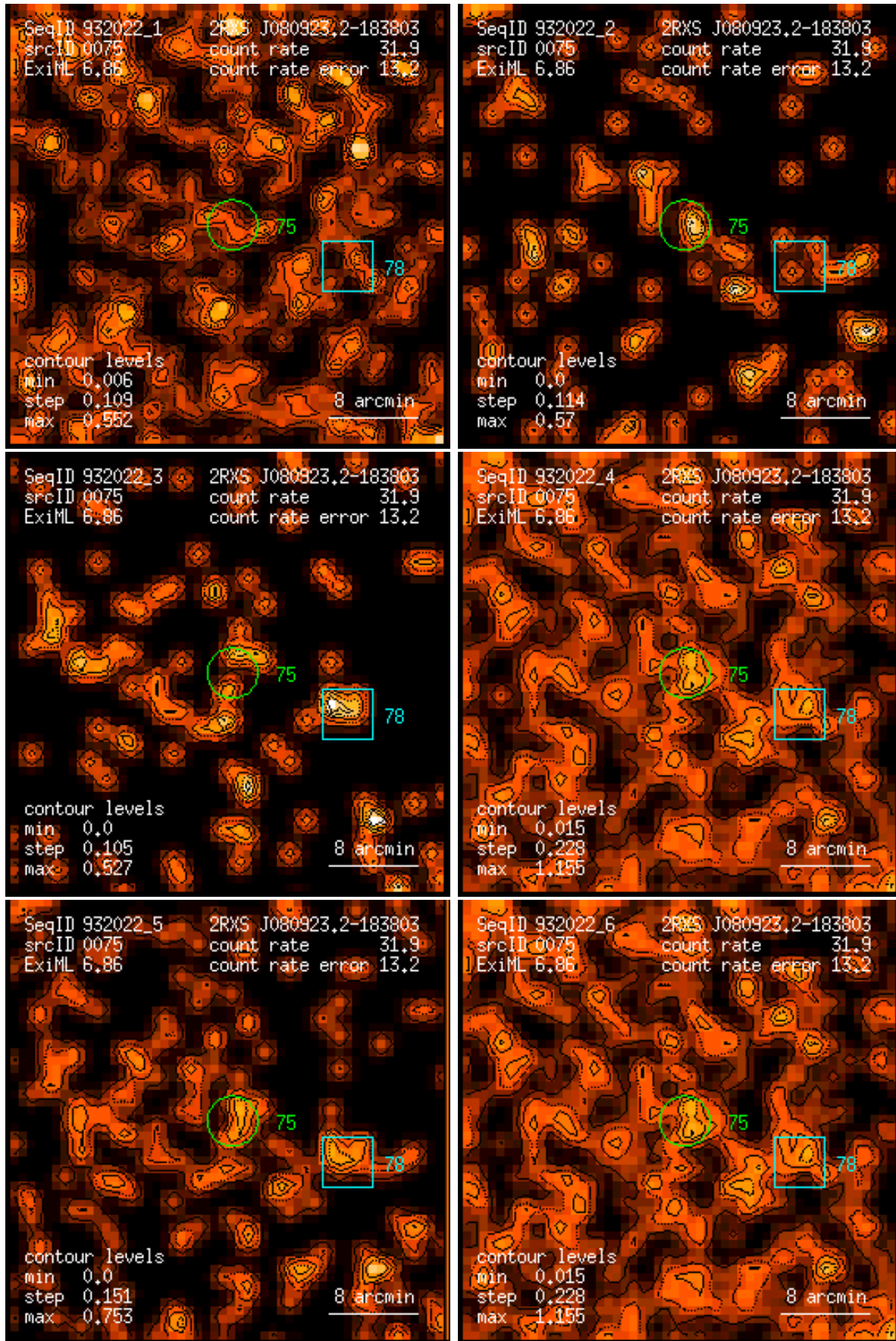
Figure 75: RASS 932022: detection 0075: band rate images, Gaussian filter: (1) PSPC channels 11 – 41, (2) 52 – 90, (3) 91 – 201, (4) 11 – 235, (5) 52 – 201, (6) 11 – 201. Broad band rates in counts/ks. Band rate contour levels in counts/ks/arcmin 2 .
