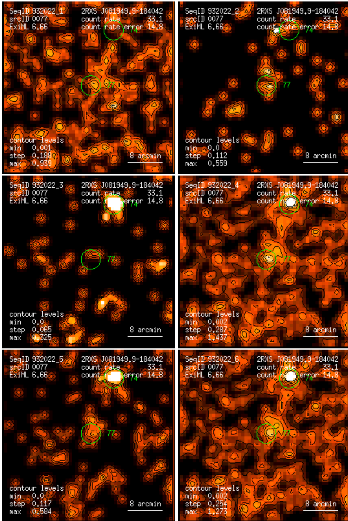
Figure 77: RASS 932022: detection 0077: band rate images, Gaussian filter: (1) PSPC channels 11 – 41, (2) 52 – 90, (3) 91 – 201, (4) 11 – 235, (5) 52 – 201, (6) 11 – 201. Broad band rates in counts/ks. Band rate contour levels in counts/ks/arcmin 2 .
