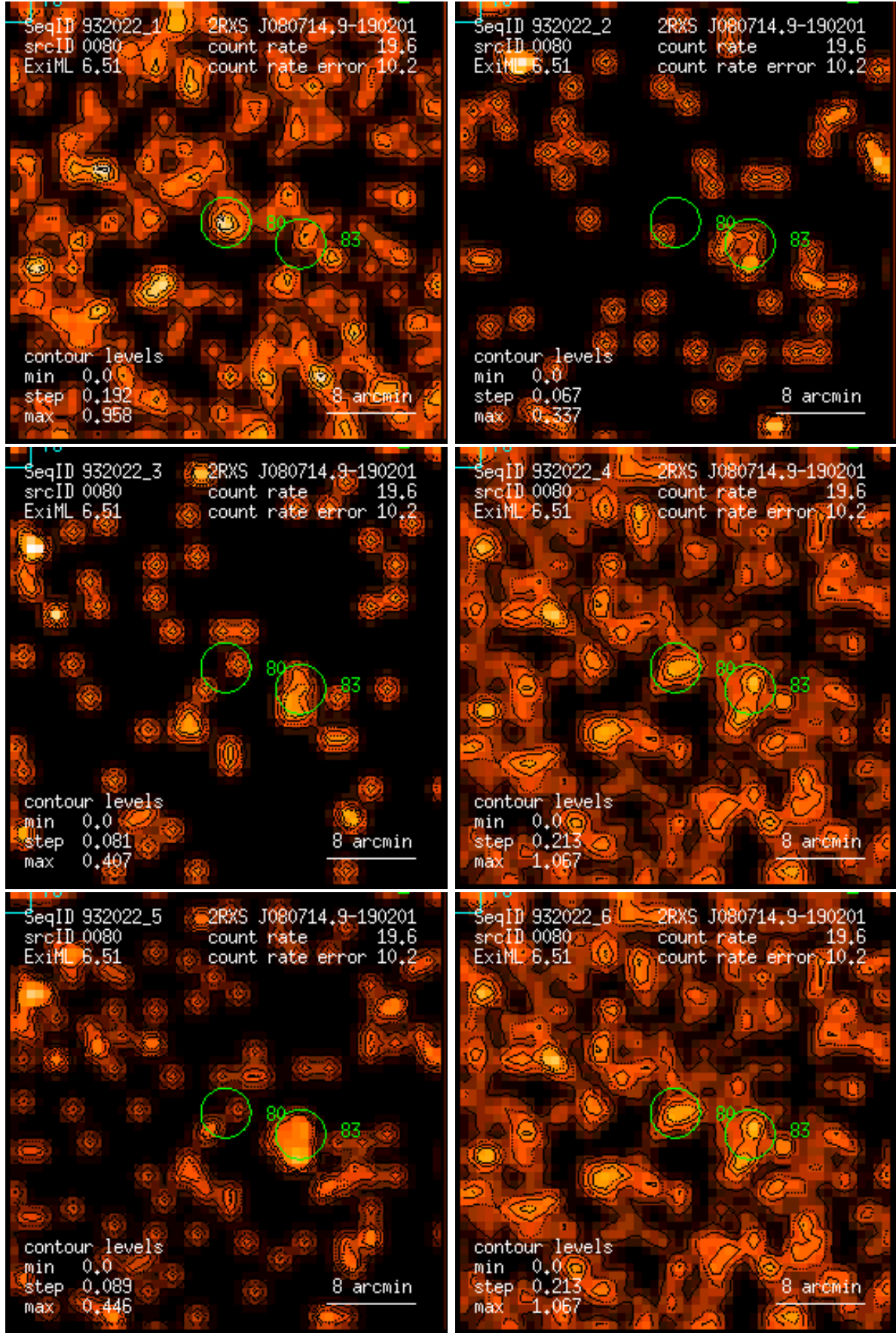
Figure 80: RASS 932022: detection 0080: band rate images, Gaussian filter: (1) PSPC channels 11 – 41, (2) 52 – 90, (3) 91 – 201, (4) 11 – 235, (5) 52 – 201, (6) 11 – 201. Broad band rates in counts/ks. Band rate contour levels in counts/ks/arcmin 2 .
