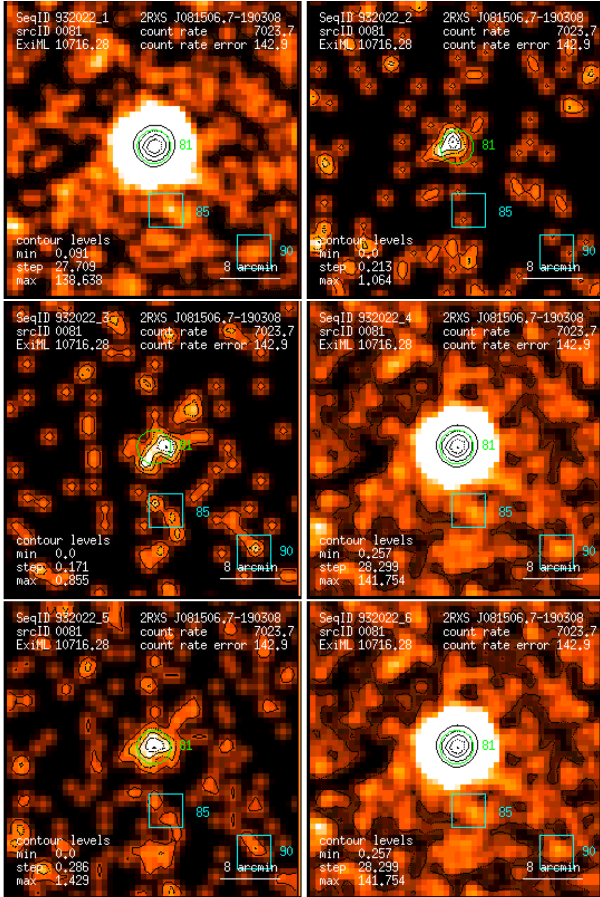
Figure 81: RASS 932022: detection 0081: band rate images, Gaussian filter: (1) PSPC channels 11 – 41, (2) 52 – 90, (3) 91 – 201, (4) 11 – 235, (5) 52 – 201, (6) 11 – 201. Broad band rates in counts/ks. Band rate contour levels in counts/ks/arcmin 2 .
