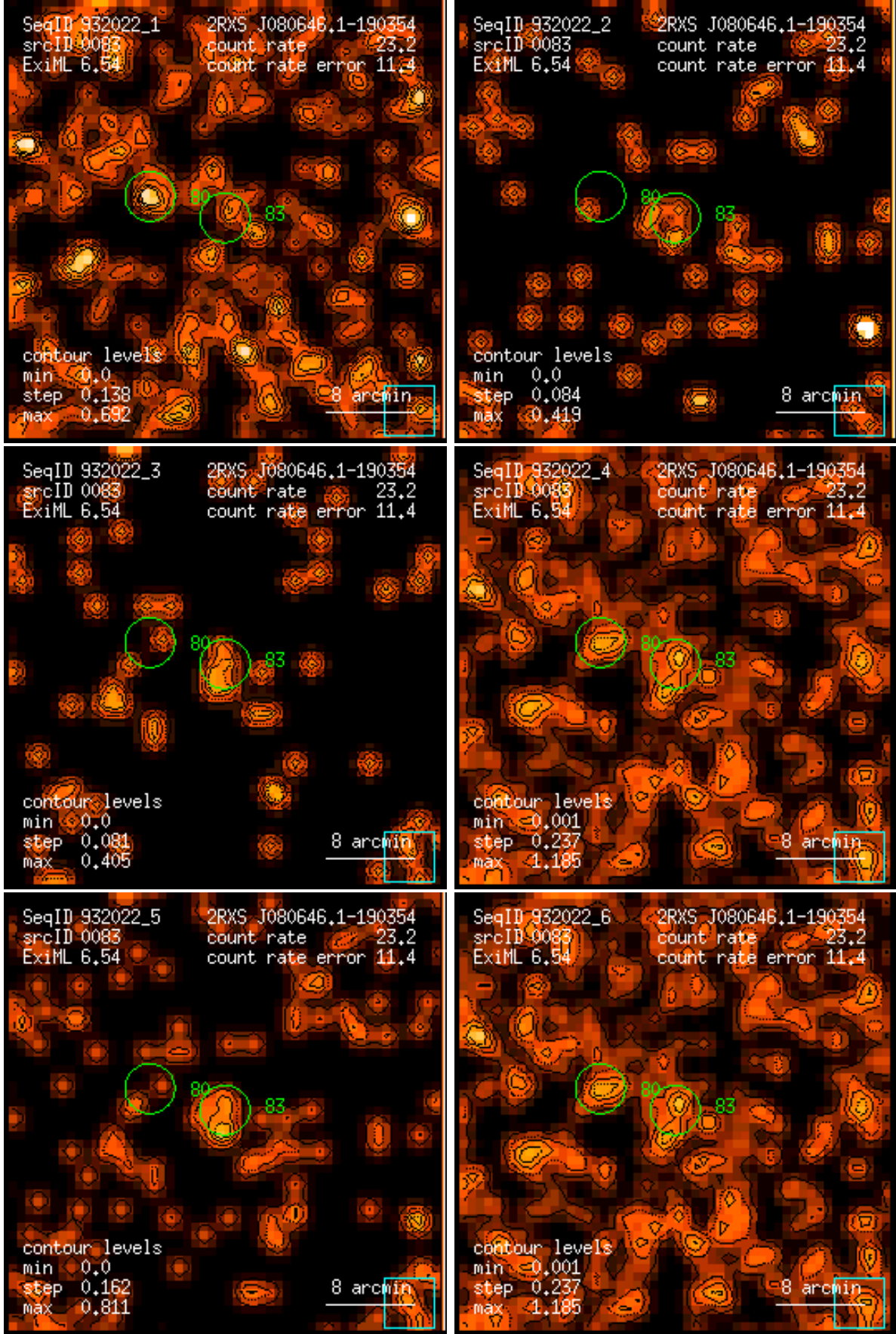
Figure 83: RASS 932022: detection 0083: band rate images, Gaussian filter: (1) PSPC channels 11 – 41, (2) 52 – 90, (3) 91 – 201, (4) 11 – 235, (5) 52 – 201, (6) 11 – 201. Broad band rates in counts/ks. Band rate contour levels in counts/ks/arcmin 2 .
