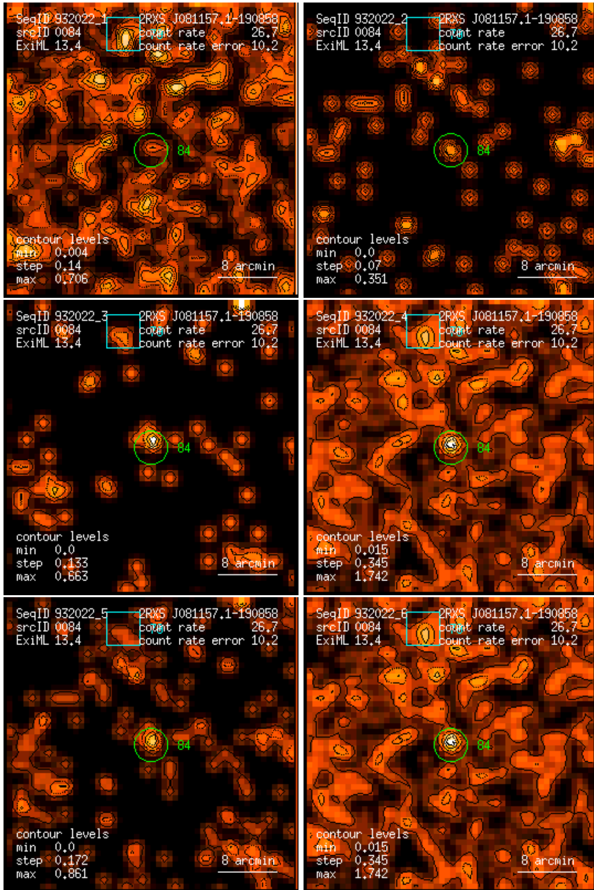
Figure 84: RASS 932022: detection 0084: band rate images, Gaussian filter: (1) PSPC channels 11 – 41, (2) 52 – 90, (3) 91 – 201, (4) 11 – 235, (5) 52 – 201, (6) 11 – 201. Broad band rates in counts/ks. Band rate contour levels in counts/ks/arcmin 2 .
