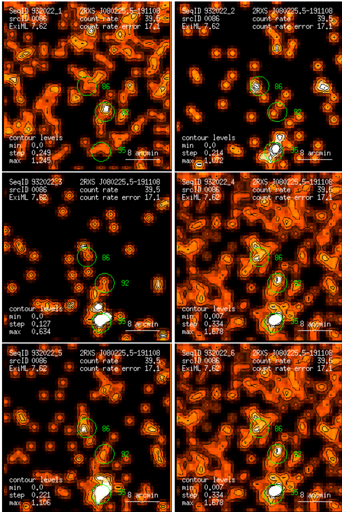
Figure 86: RASS 932022: detection 0086: band rate images, Gaussian filter: (1) PSPC channels 11 – 41, (2) 52 – 90, (3) 91 – 201, (4) 11 – 235, (5) 52 – 201, (6) 11 – 201. Broad band rates in counts/ks. Band rate contour levels in counts/ks/arcmin 2 .
