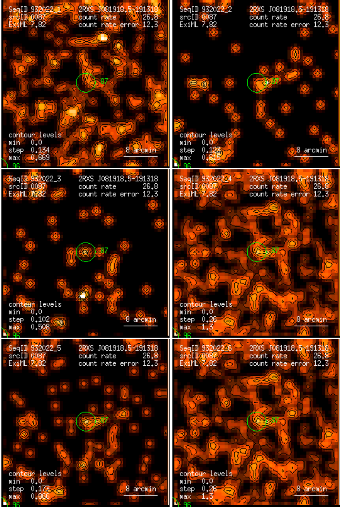
Figure 87: RASS 932022: detection 0087: band rate images, Gaussian filter: (1) PSPC channels 11 – 41, (2) 52 – 90, (3) 91 – 201, (4) 11 – 235, (5) 52 – 201, (6) 11 – 201. Broad band rates in counts/ks. Band rate contour levels in counts/ks/arcmin 2 .
