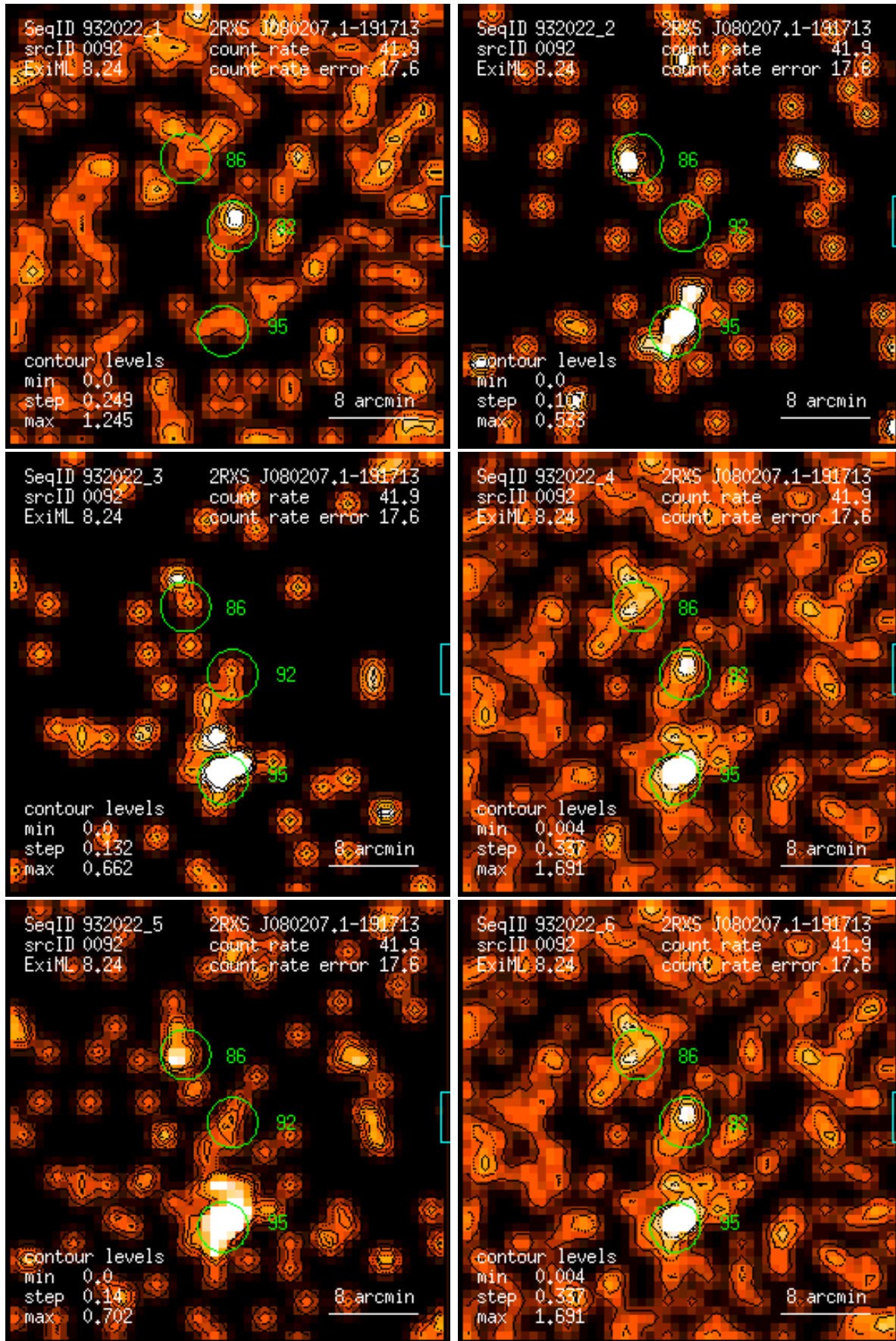
Figure 92: RASS 932022: detection 0092: band rate images, Gaussian filter: (1) PSPC channels 11 – 41, (2) 52 – 90, (3) 91 – 201, (4) 11 – 235, (5) 52 – 201, (6) 11 – 201. Broad band rates in counts/ks. Band rate contour levels in counts/ks/arcmin 2 .
