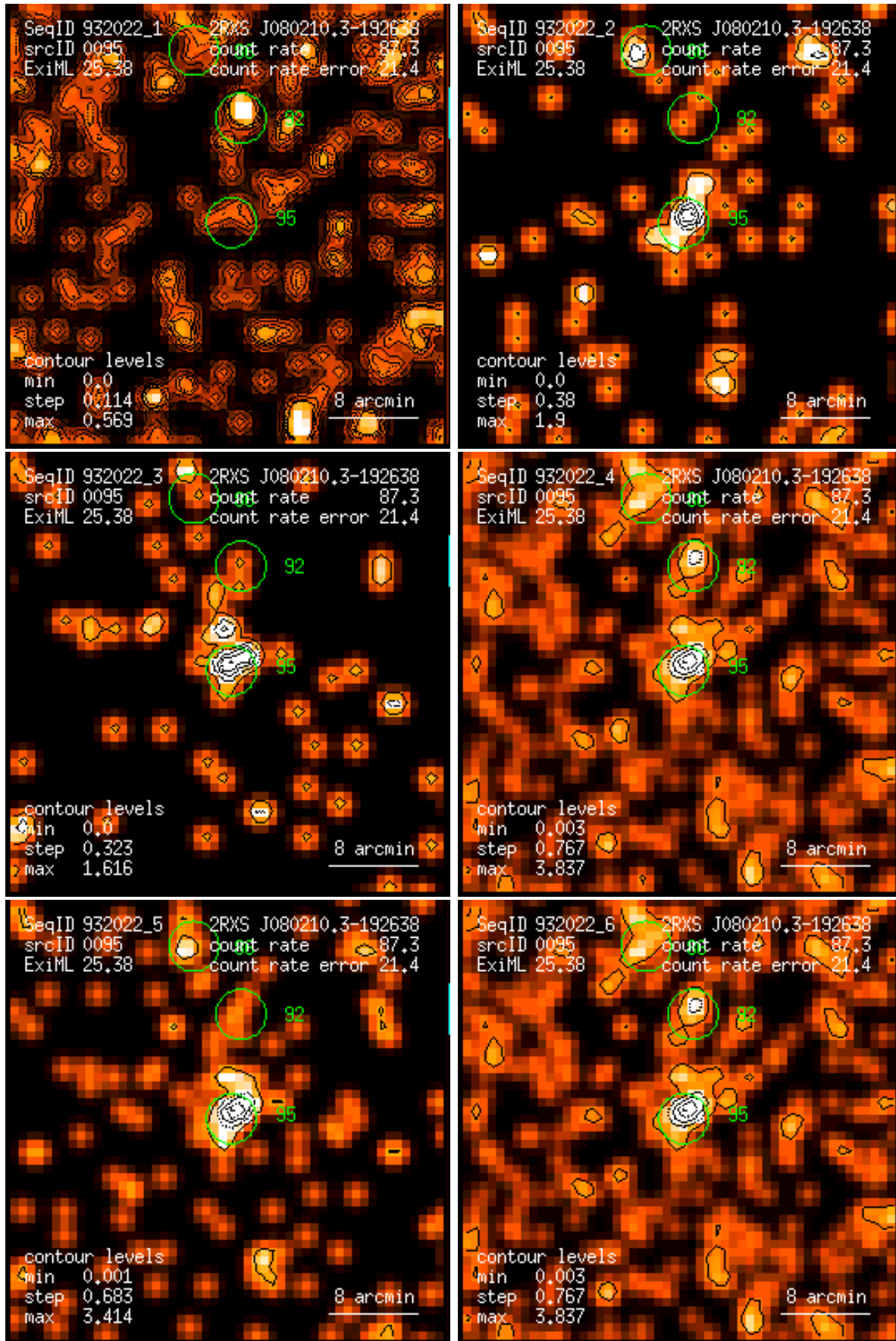
Figure 95: RASS 932022: detection 0095: band rate images, Gaussian filter: (1) PSPC channels 11 – 41, (2) 52 – 90, (3) 91 – 201, (4) 11 – 235, (5) 52 – 201, (6) 11 – 201. Broad band rates in counts/ks. Band rate contour levels in counts/ks/arcmin 2 .
