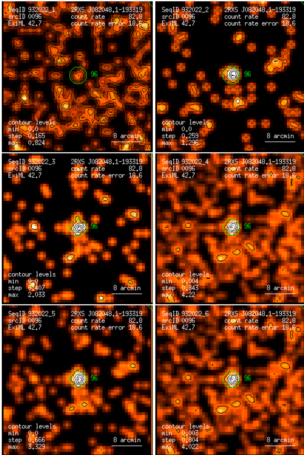
Figure 96: RASS 932022: detection 0096: band rate images, Gaussian filter: (1) PSPC channels 11 – 41, (2) 52 – 90, (3) 91 – 201, (4) 11 – 235, (5) 52 – 201, (6) 11 – 201. Broad band rates in counts/ks. Band rate contour levels in counts/ks/arcmin 2 .
