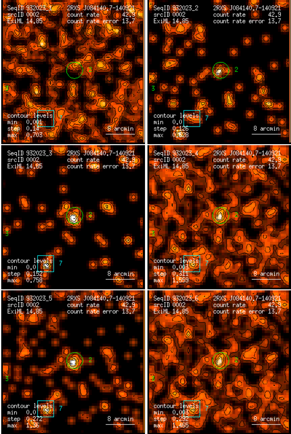
Figure 2: RASS 932023: detection 0002: band rate images, Gaussian filter: (1) PSPC channels 11 – 41, (2) 52 – 90, (3) 91 – 201, (4) 11 – 235, (5) 52 – 201, (6) 11 – 201. Broad band rates in counts/ks. Band rate contour levels in counts/ks/arcmin 2 .
