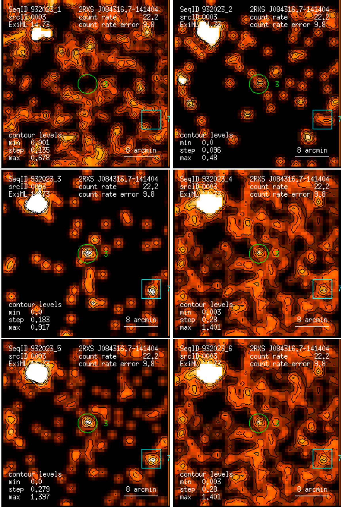
Figure 3: RASS 932023: detection 0003: band rate images, Gaussian filter: (1) PSPC channels 11 – 41, (2) 52 – 90, (3) 91 – 201, (4) 11 – 235, (5) 52 – 201, (6) 11 – 201. Broad band rates in counts/ks. Band rate contour levels in counts/ks/arcmin 2 .
