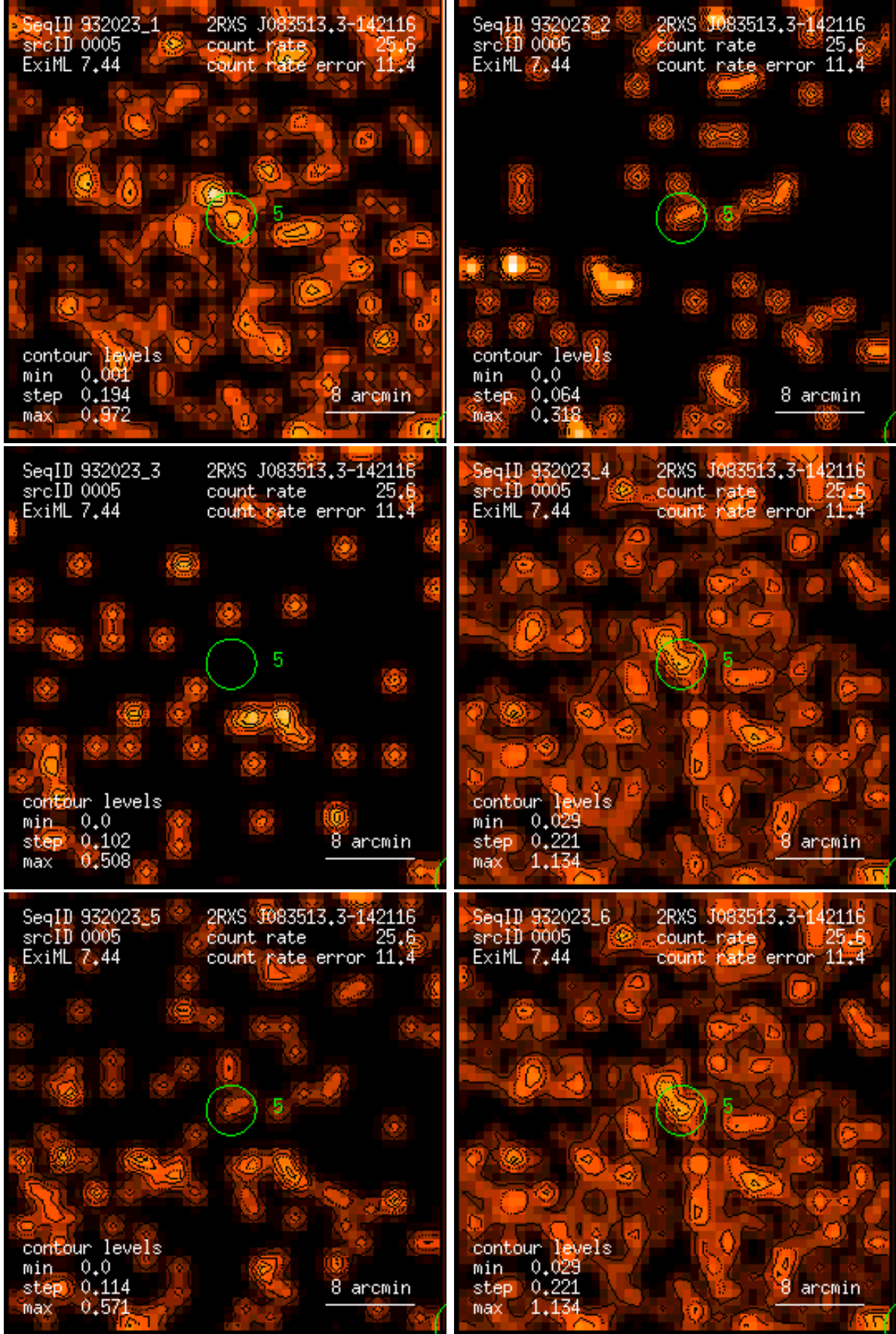
Figure 5: RASS 932023: detection 0005: band rate images, Gaussian filter: (1) PSPC channels 11 – 41, (2) 52 – 90, (3) 91 – 201, (4) 11 – 235, (5) 52 – 201, (6) 11 – 201. Broad band rates in counts/ks. Band rate contour levels in counts/ks/arcmin 2 .
