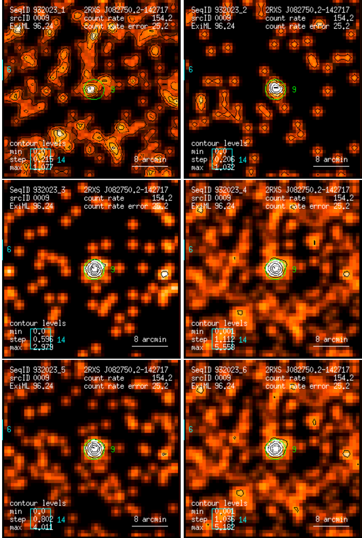
Figure 9: RASS 932023: detection 0009: band rate images, Gaussian filter: (1) PSPC channels 11 – 41, (2) 52 – 90, (3) 91 – 201, (4) 11 – 235, (5) 52 – 201, (6) 11 – 201. Broad band rates in counts/ks. Band rate contour levels in counts/ks/arcmin 2 .
