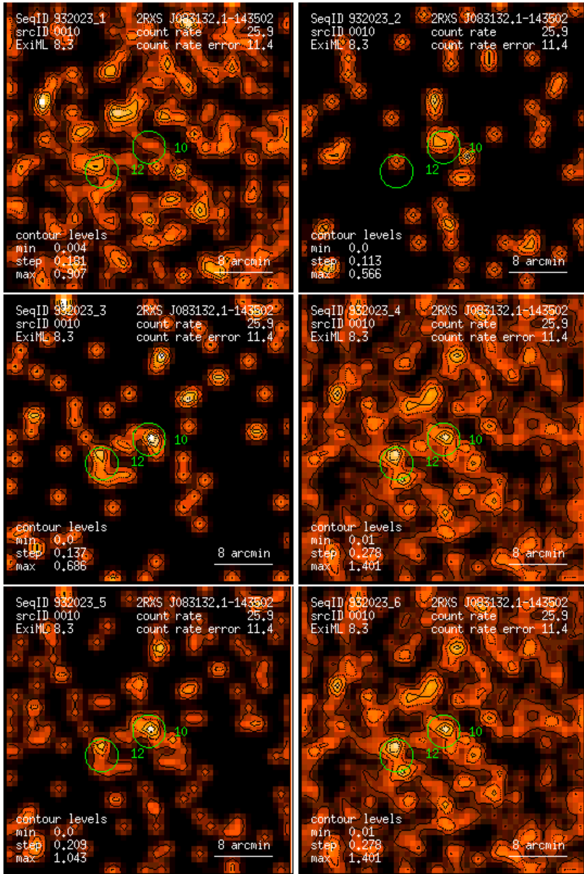
Figure 10: RASS 932023: detection 0010: band rate images, Gaussian filter: (1) PSPC channels 11 – 41, (2) 52 – 90, (3) 91 – 201, (4) 11 – 235, (5) 52 – 201, (6) 11 – 201. Broad band rates in counts/ks. Band rate contour levels in counts/ks/arcmin 2 .
