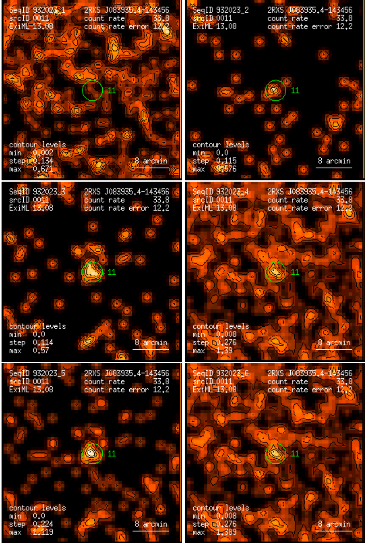
Figure 11: RASS 932023: detection 0011: band rate images, Gaussian filter: (1) PSPC channels 11 – 41, (2) 52 – 90, (3) 91 – 201, (4) 11 – 235, (5) 52 – 201, (6) 11 – 201. Broad band rates in counts/ks. Band rate contour levels in counts/ks/arcmin 2 .
