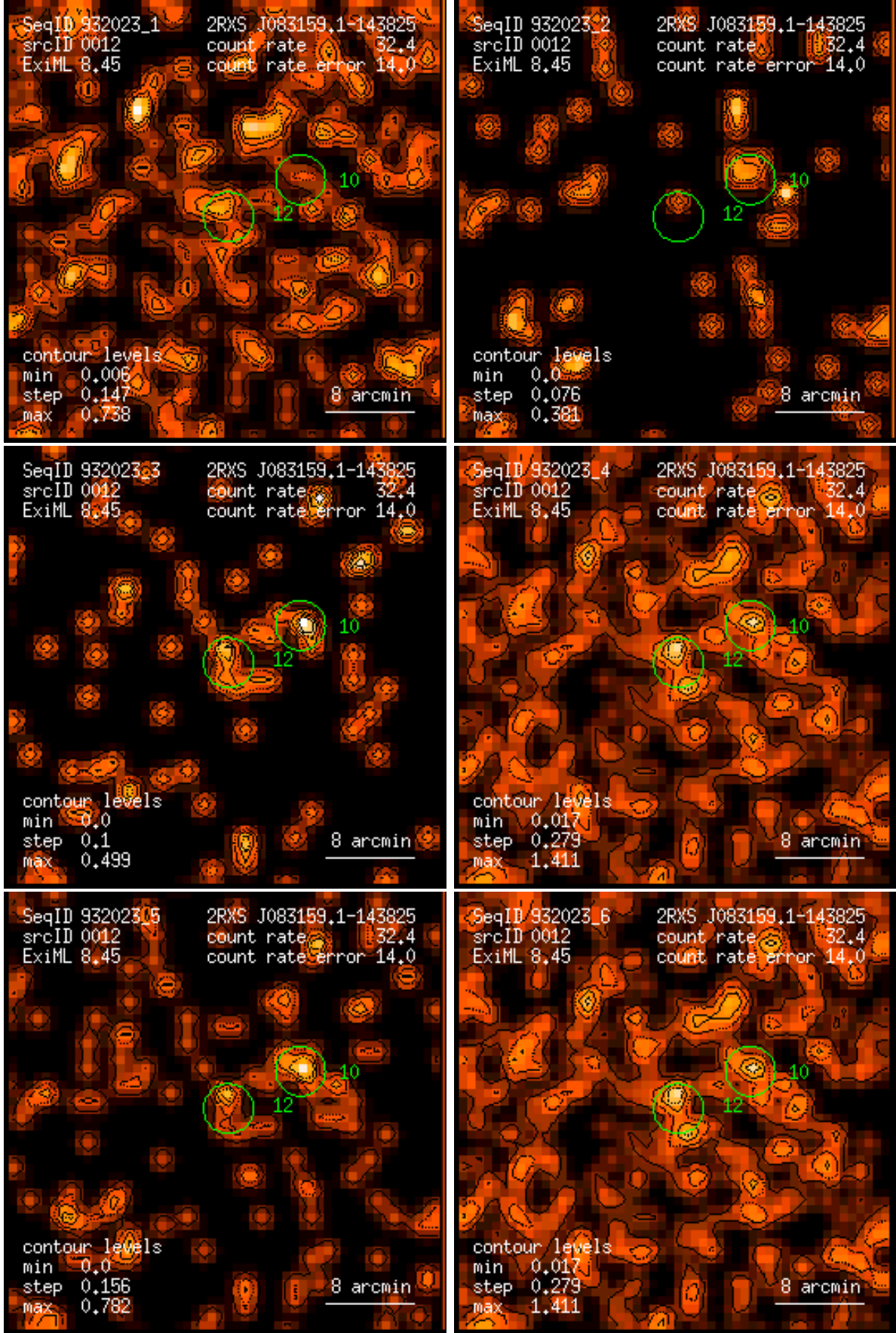
Figure 12: RASS 932023: detection 0012: band rate images, Gaussian filter: (1) PSPC channels 11 – 41, (2) 52 – 90, (3) 91 – 201, (4) 11 – 235, (5) 52 – 201, (6) 11 – 201. Broad band rates in counts/ks. Band rate contour levels in counts/ks/arcmin 2 .
