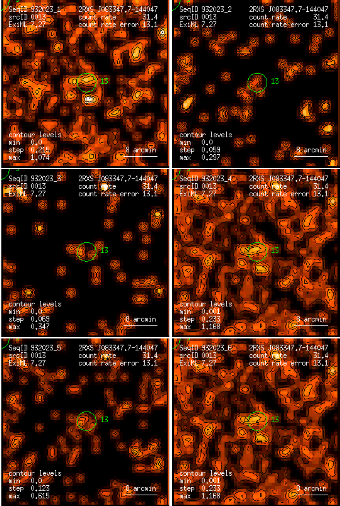
Figure 13: RASS 932023: detection 0013: band rate images, Gaussian filter: (1) PSPC channels 11 – 41, (2) 52 – 90, (3) 91 – 201, (4) 11 – 235, (5) 52 – 201, (6) 11 – 201. Broad band rates in counts/ks. Band rate contour levels in counts/ks/arcmin 2 .
