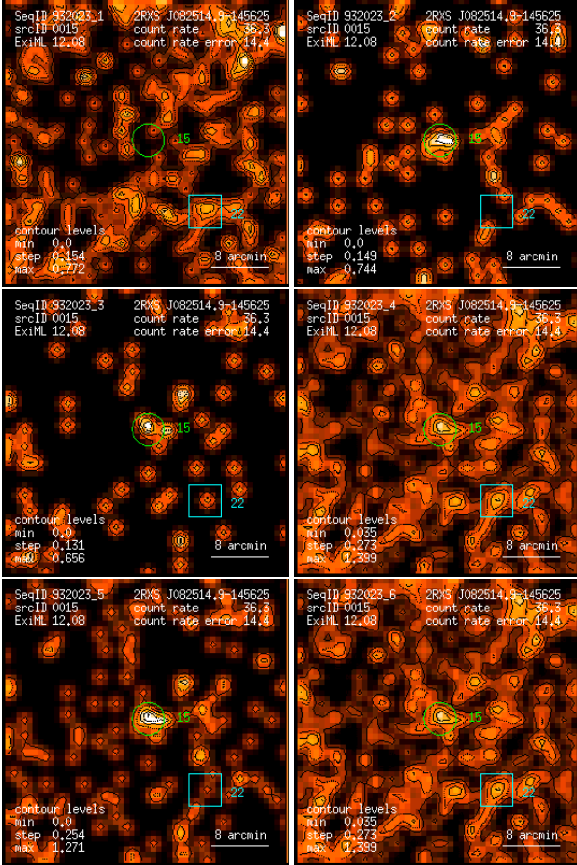
Figure 15: RASS 932023: detection 0015: band rate images, Gaussian filter: (1) PSPC channels 11 – 41, (2) 52 – 90, (3) 91 – 201, (4) 11 – 235, (5) 52 – 201, (6) 11 – 201. Broad band rates in counts/ks. Band rate contour levels in counts/ks/arcmin 2 .
