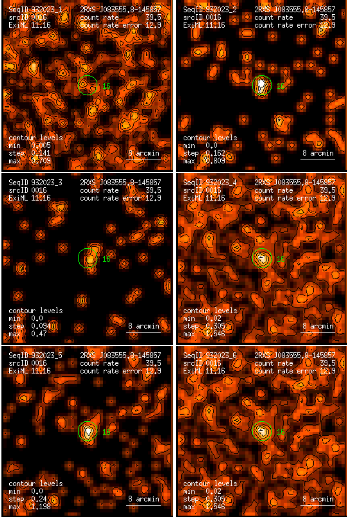
Figure 16: RASS 932023: detection 0016: band rate images, Gaussian filter: (1) PSPC channels 11 – 41, (2) 52 – 90, (3) 91 – 201, (4) 11 – 235, (5) 52 – 201, (6) 11 – 201. Broad band rates in counts/ks. Band rate contour levels in counts/ks/arcmin 2 .
