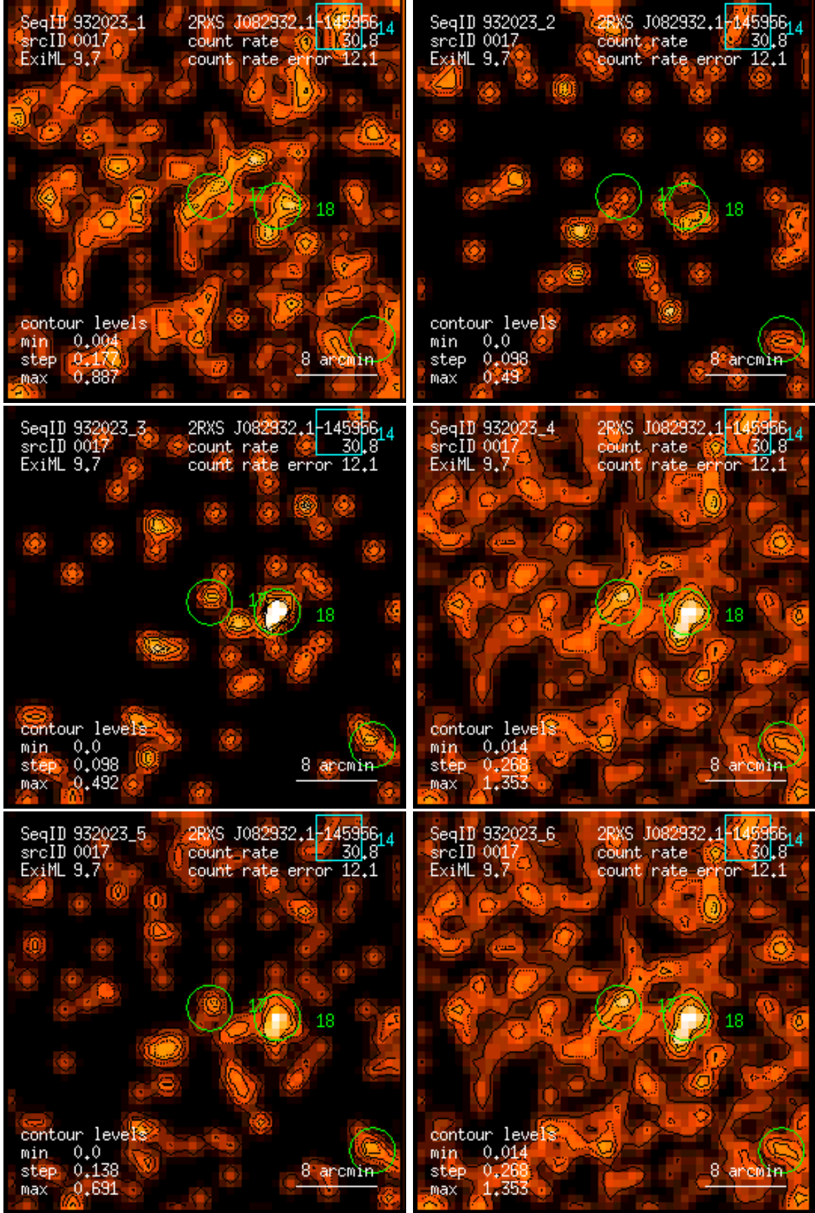
Figure 17: RASS 932023: detection 0017: band rate images, Gaussian filter: (1) PSPC channels 11 – 41, (2) 52 – 90, (3) 91 – 201, (4) 11 – 235, (5) 52 – 201, (6) 11 – 201. Broad band rates in counts/ks. Band rate contour levels in counts/ks/arcmin 2 .
