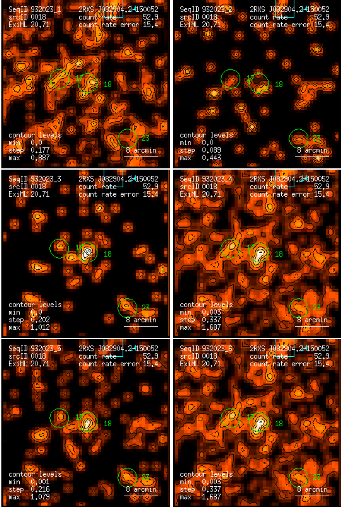
Figure 18: RASS 932023: detection 0018: band rate images, Gaussian filter: (1) PSPC channels 11 – 41, (2) 52 – 90, (3) 91 – 201, (4) 11 – 235, (5) 52 – 201, (6) 11 – 201. Broad band rates in counts/ks. Band rate contour levels in counts/ks/arcmin 2 .
