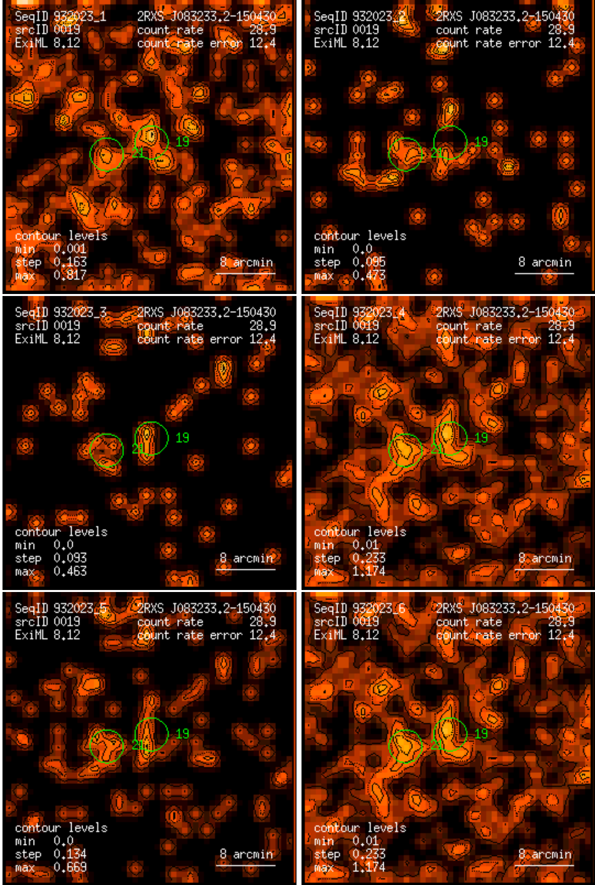
Figure 19: RASS 932023: detection 0019: band rate images, Gaussian filter: (1) PSPC channels 11 – 41, (2) 52 – 90, (3) 91 – 201, (4) 11 – 235, (5) 52 – 201, (6) 11 – 201. Broad band rates in counts/ks. Band rate contour levels in counts/ks/arcmin 2 .
