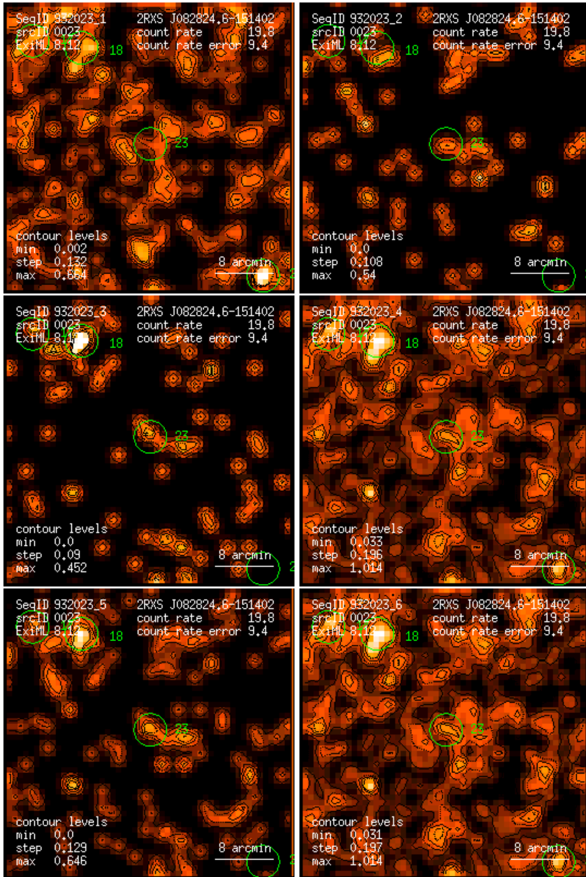
Figure 23: RASS 932023: detection 0023: band rate images, Gaussian filter: (1) PSPC channels 11 – 41, (2) 52 – 90, (3) 91 – 201, (4) 11 – 235, (5) 52 – 201, (6) 11 – 201. Broad band rates in counts/ks. Band rate contour levels in counts/ks/arcmin 2 .
