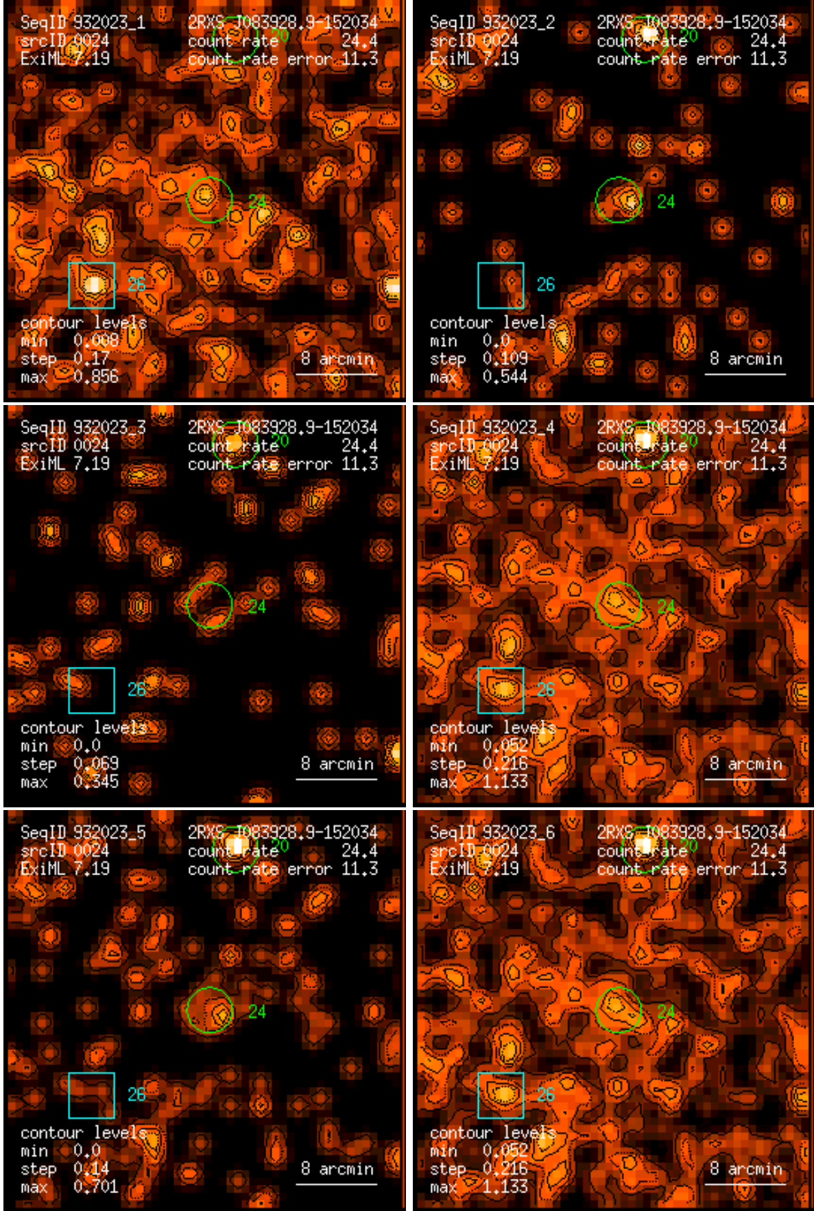
Figure 24: RASS 932023: detection 0024: band rate images, Gaussian filter: (1) PSPC channels 11 – 41, (2) 52 – 90, (3) 91 – 201, (4) 11 – 235, (5) 52 – 201, (6) 11 – 201. Broad band rates in counts/ks. Band rate contour levels in counts/ks/arcmin 2 .
