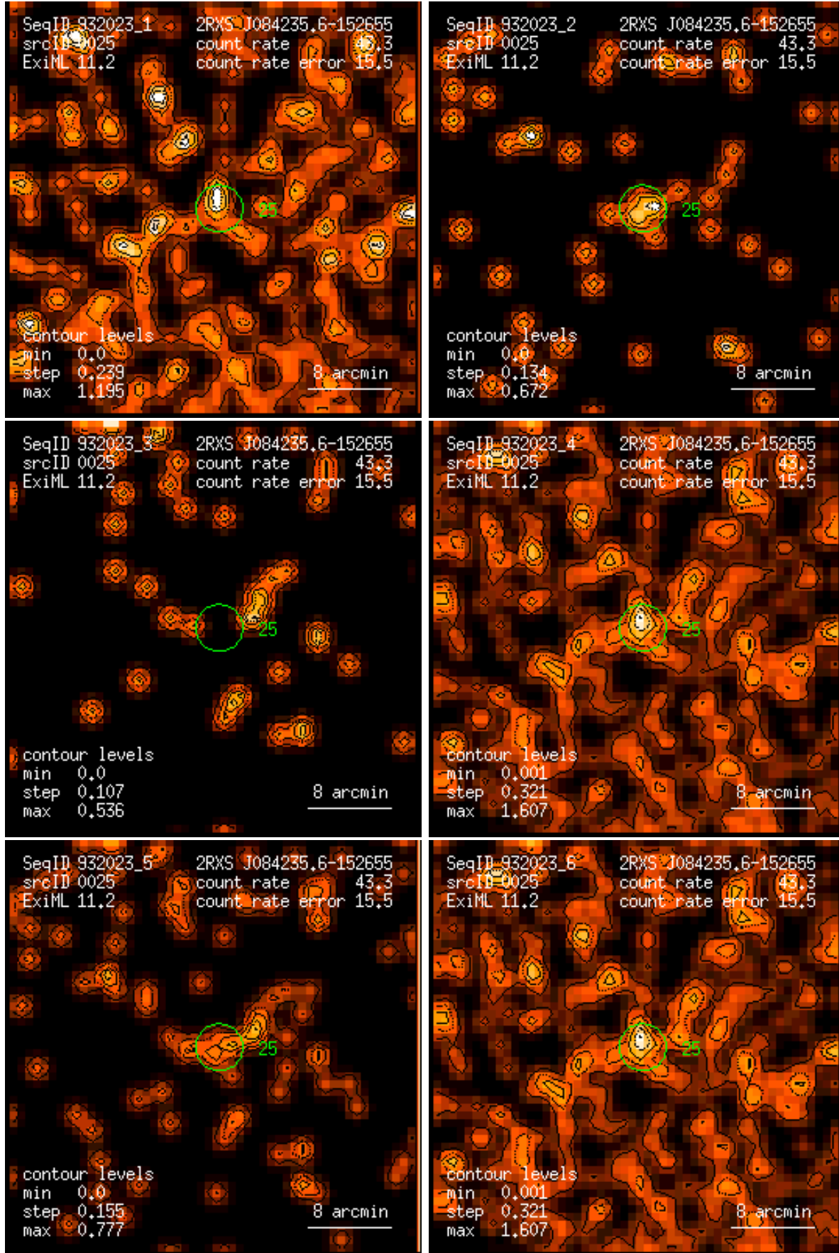
Figure 25: RASS 932023: detection 0025: band rate images, Gaussian filter: (1) PSPC channels 11 – 41, (2) 52 – 90, (3) 91 – 201, (4) 11 – 235, (5) 52 – 201, (6) 11 – 201. Broad band rates in counts/ks. Band rate contour levels in counts/ks/arcmin 2 .
