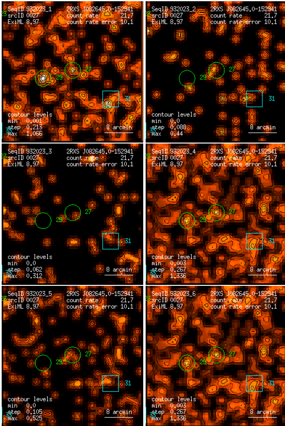
Figure 27: RASS 932023: detection 0027: band rate images, Gaussian filter: (1) PSPC channels 11 – 41, (2) 52 – 90, (3) 91 – 201, (4) 11 – 235, (5) 52 – 201, (6) 11 – 201. Broad band rates in counts/ks. Band rate contour levels in counts/ks/arcmin 2 .
