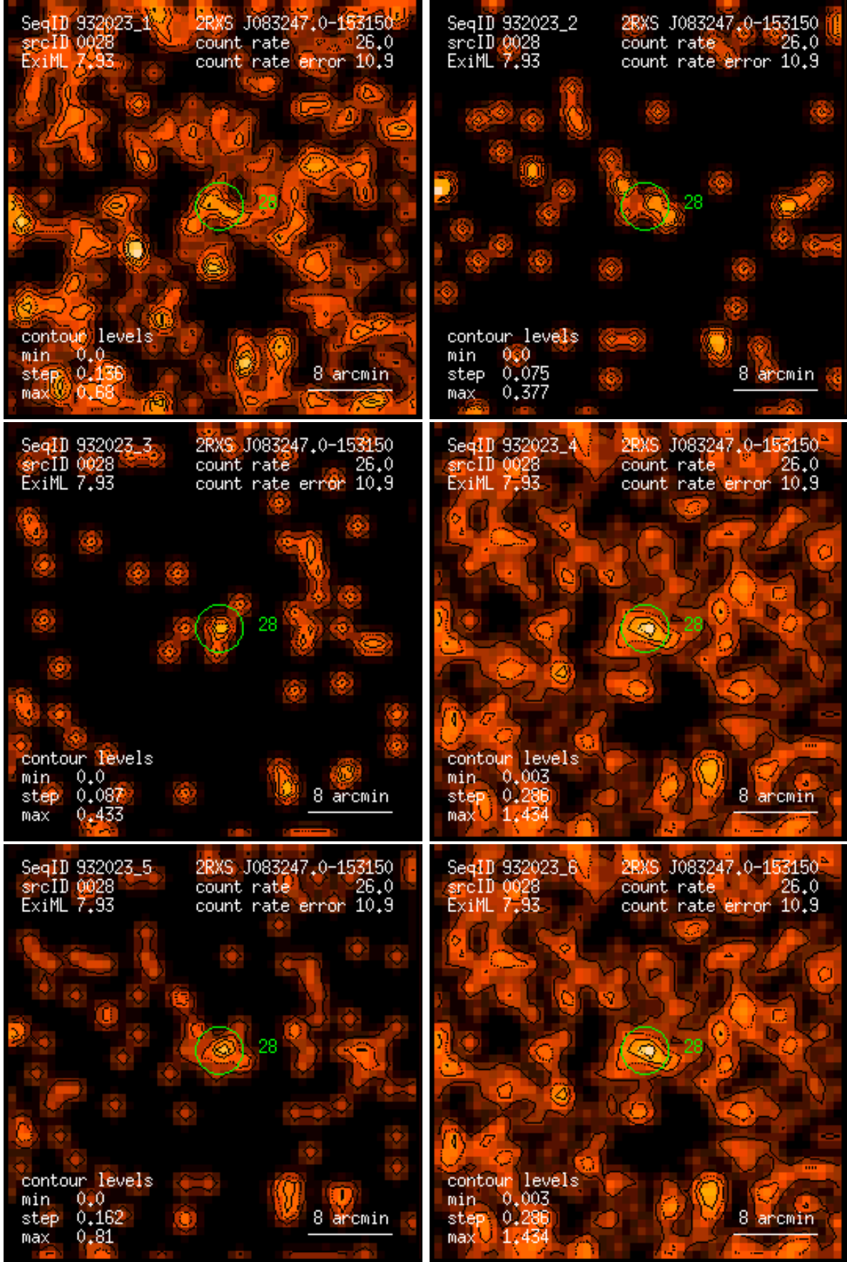
Figure 28: RASS 932023: detection 0028: band rate images, Gaussian filter: (1) PSPC channels 11 – 41, (2) 52 – 90, (3) 91 – 201, (4) 11 – 235, (5) 52 – 201, (6) 11 – 201. Broad band rates in counts/ks. Band rate contour levels in counts/ks/arcmin 2 .
