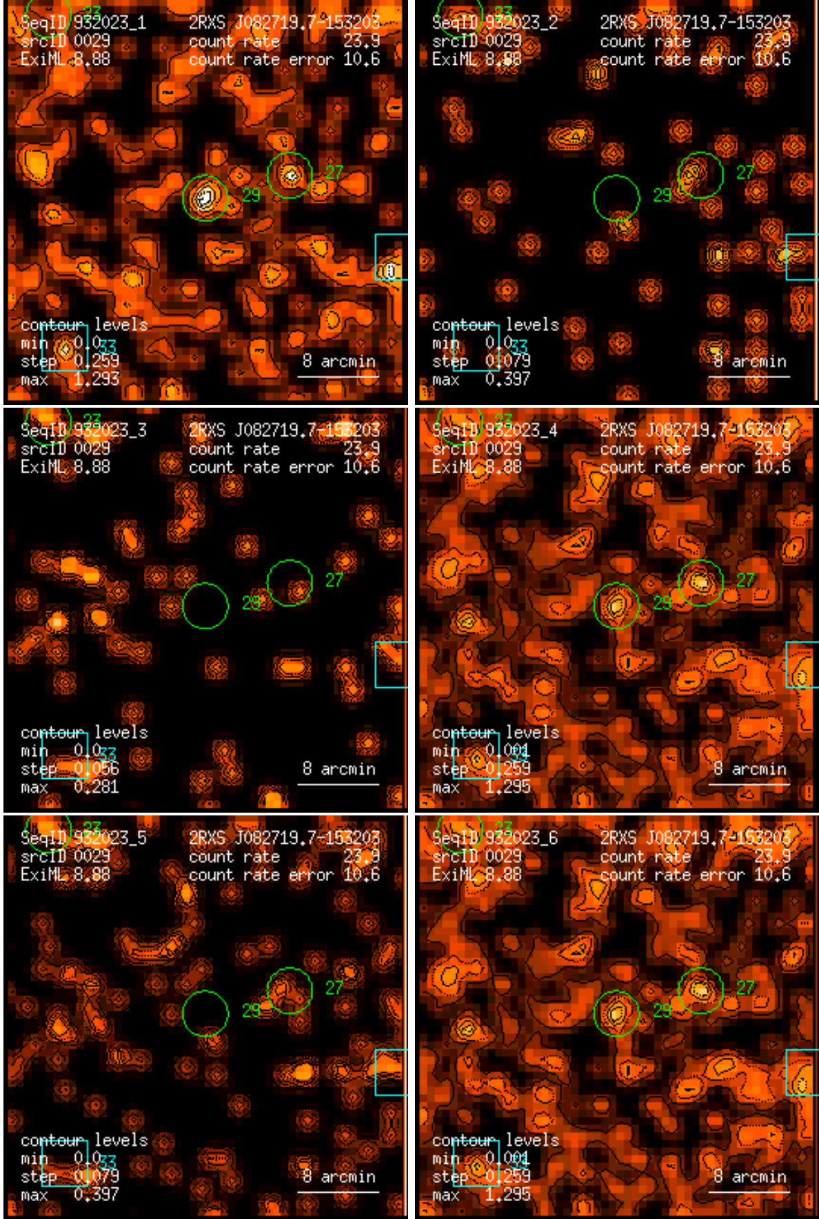
Figure 29: RASS 932023: detection 0029: band rate images, Gaussian filter: (1) PSPC channels 11 – 41, (2) 52 – 90, (3) 91 – 201, (4) 11 – 235, (5) 52 – 201, (6) 11 – 201. Broad band rates in counts/ks. Band rate contour levels in counts/ks/arcmin 2 .
