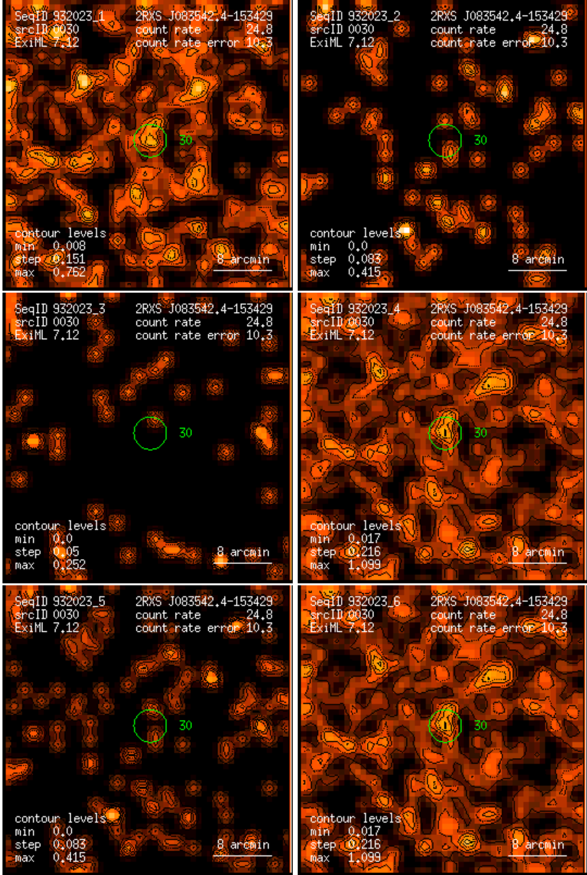
Figure 30: RASS 932023: detection 0030: band rate images, Gaussian filter: (1) PSPC channels 11 – 41, (2) 52 – 90, (3) 91 – 201, (4) 11 – 235, (5) 52 – 201, (6) 11 – 201. Broad band rates in counts/ks. Band rate contour levels in counts/ks/arcmin 2 .
