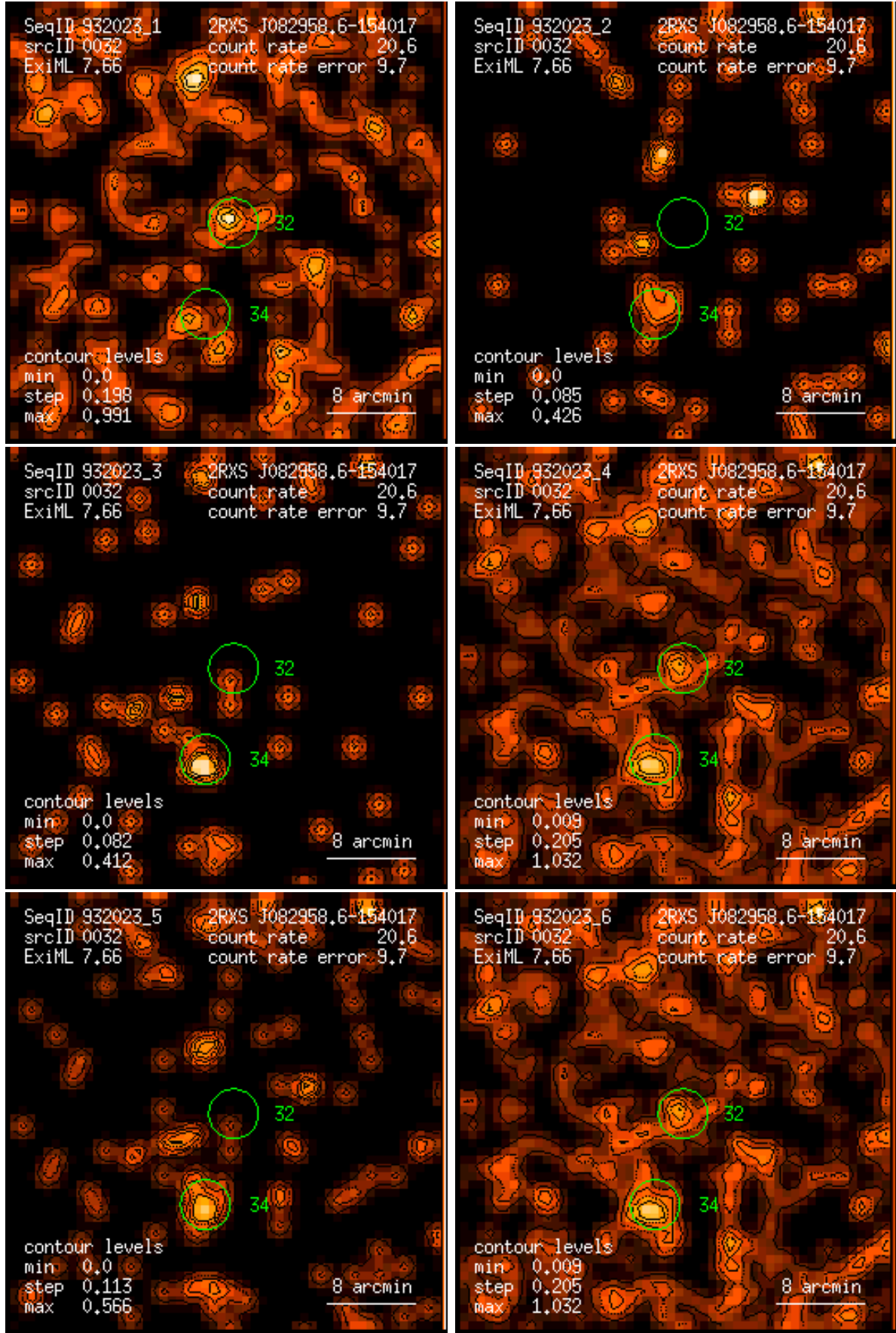
Figure 32: RASS 932023: detection 0032: band rate images, Gaussian filter: (1) PSPC channels 11 – 41, (2) 52 – 90, (3) 91 – 201, (4) 11 – 235, (5) 52 – 201, (6) 11 – 201. Broad band rates in counts/ks. Band rate contour levels in counts/ks/arcmin 2 .
