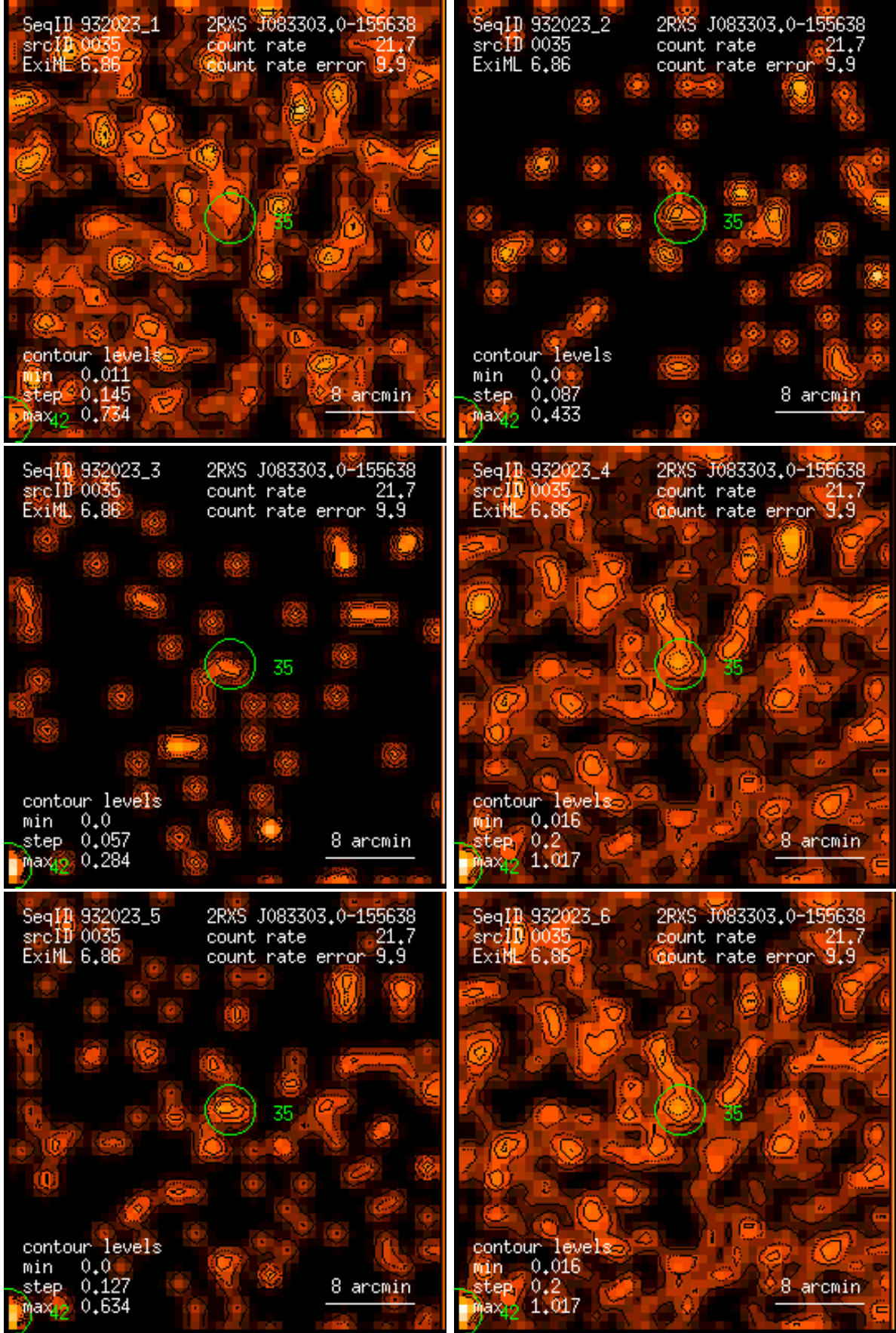
Figure 35: RASS 932023: detection 0035: band rate images, Gaussian filter: (1) PSPC channels 11 – 41, (2) 52 – 90, (3) 91 – 201, (4) 11 – 235, (5) 52 – 201, (6) 11 – 201. Broad band rates in counts/ks. Band rate contour levels in counts/ks/arcmin 2 .
