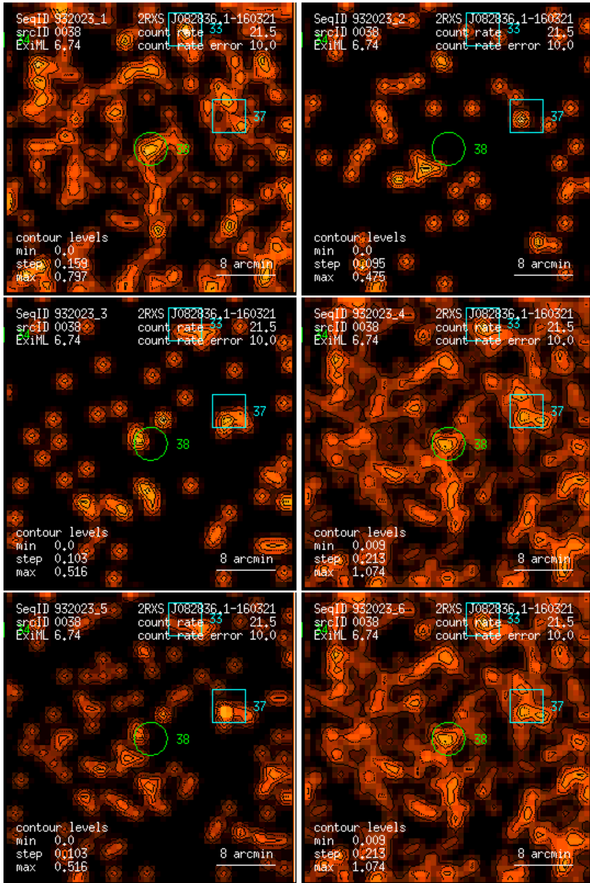
Figure 38: RASS 932023: detection 0038: band rate images, Gaussian filter: (1) PSPC channels 11 – 41, (2) 52 – 90, (3) 91 – 201, (4) 11 – 235, (5) 52 – 201, (6) 11 – 201. Broad band rates in counts/ks. Band rate contour levels in counts/ks/arcmin 2 .
