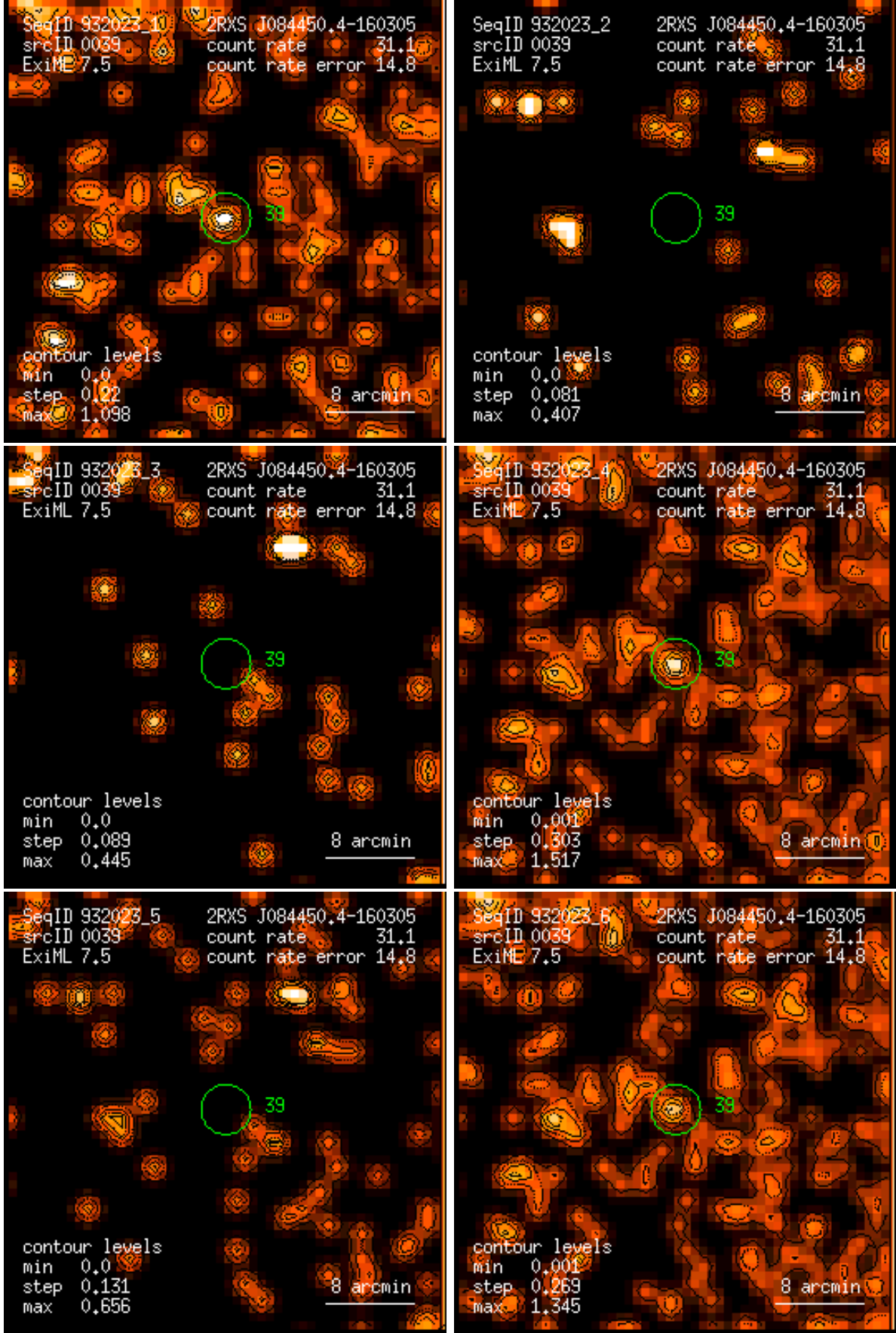
Figure 39: RASS 932023: detection 0039: band rate images, Gaussian filter: (1) PSPC channels 11 – 41, (2) 52 – 90, (3) 91 – 201, (4) 11 – 235, (5) 52 – 201, (6) 11 – 201. Broad band rates in counts/ks. Band rate contour levels in counts/ks/arcmin 2 .
